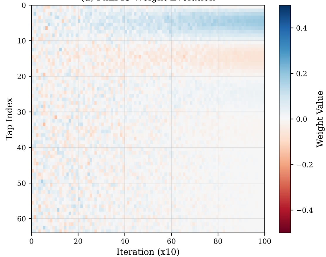
(a) FxLMS Weight Evolution
