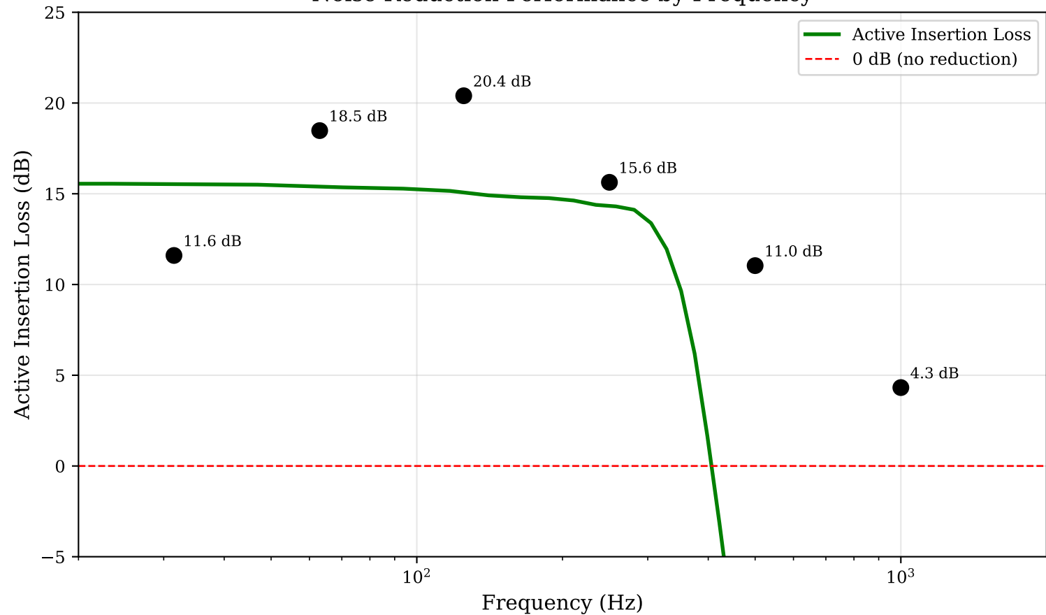
Noise Reduction Performance by Frequency
