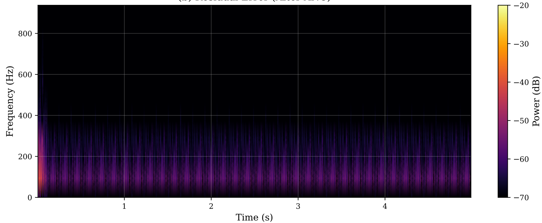
(b) Residual Error (After ANC)
