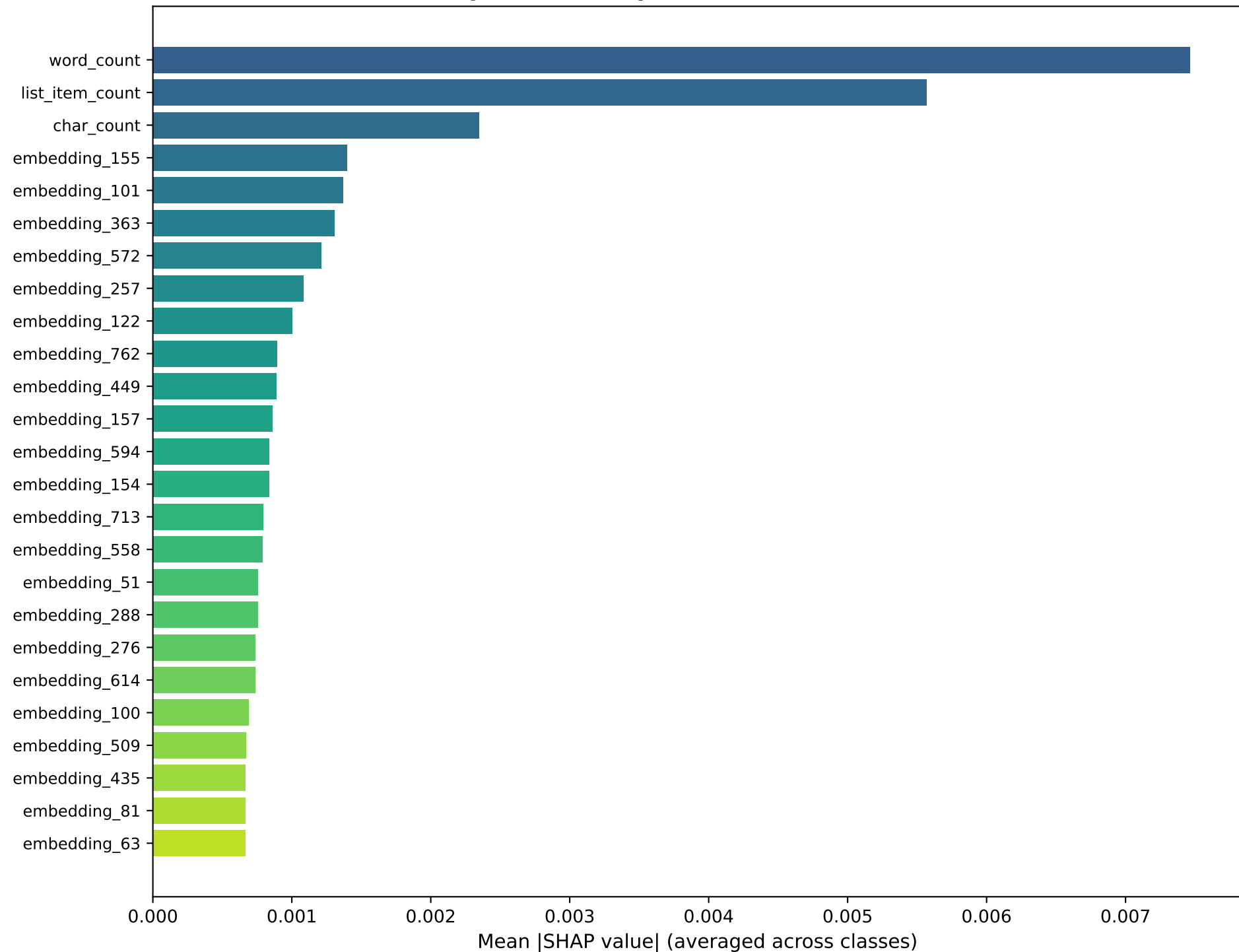
Top 25 Most Important Features (SHAP)
