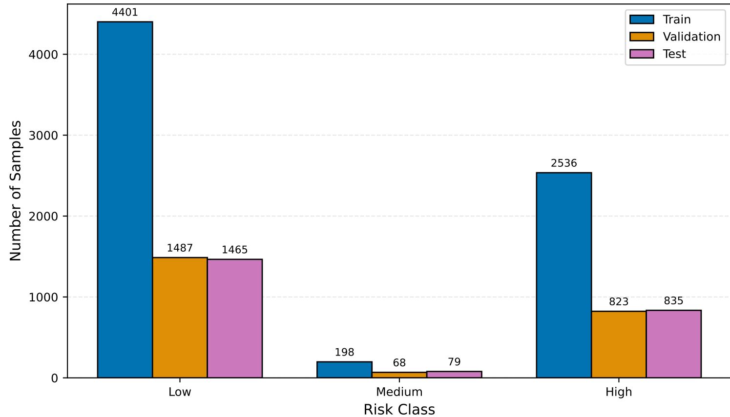
Class Distribution Across Data Splits
