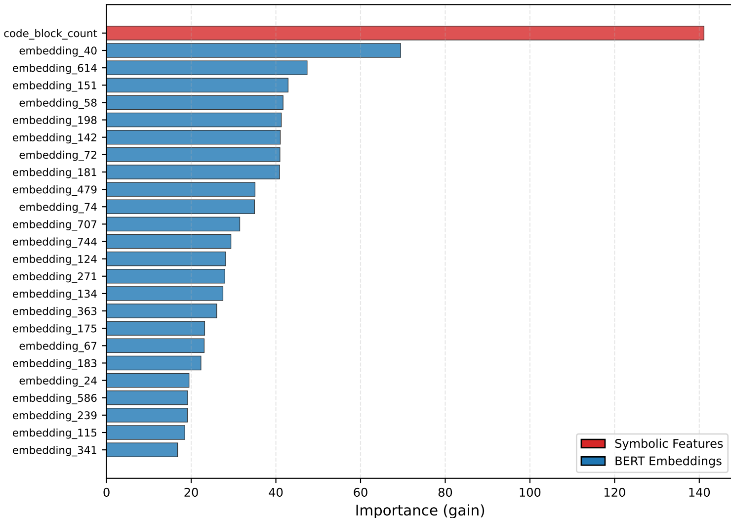
Top 25 Feature Importance
