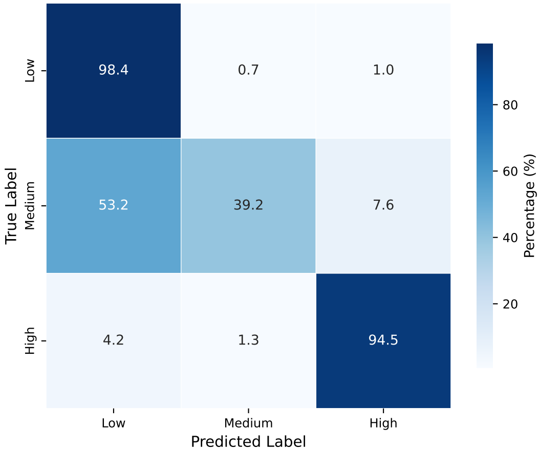
Confusion Matrix
