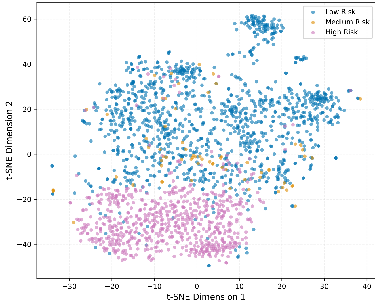
t-SNE Visualization of DistilBERT Embeddings
