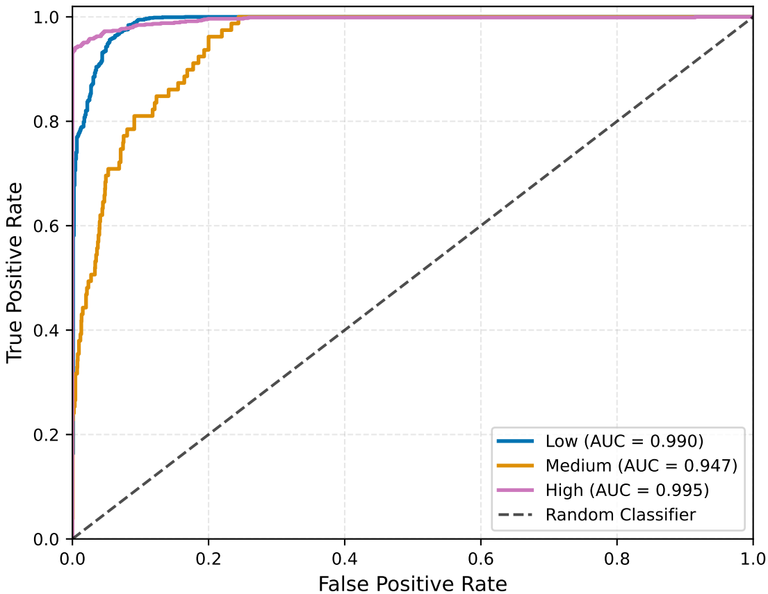
ROC Curves (One-vs-Rest)
