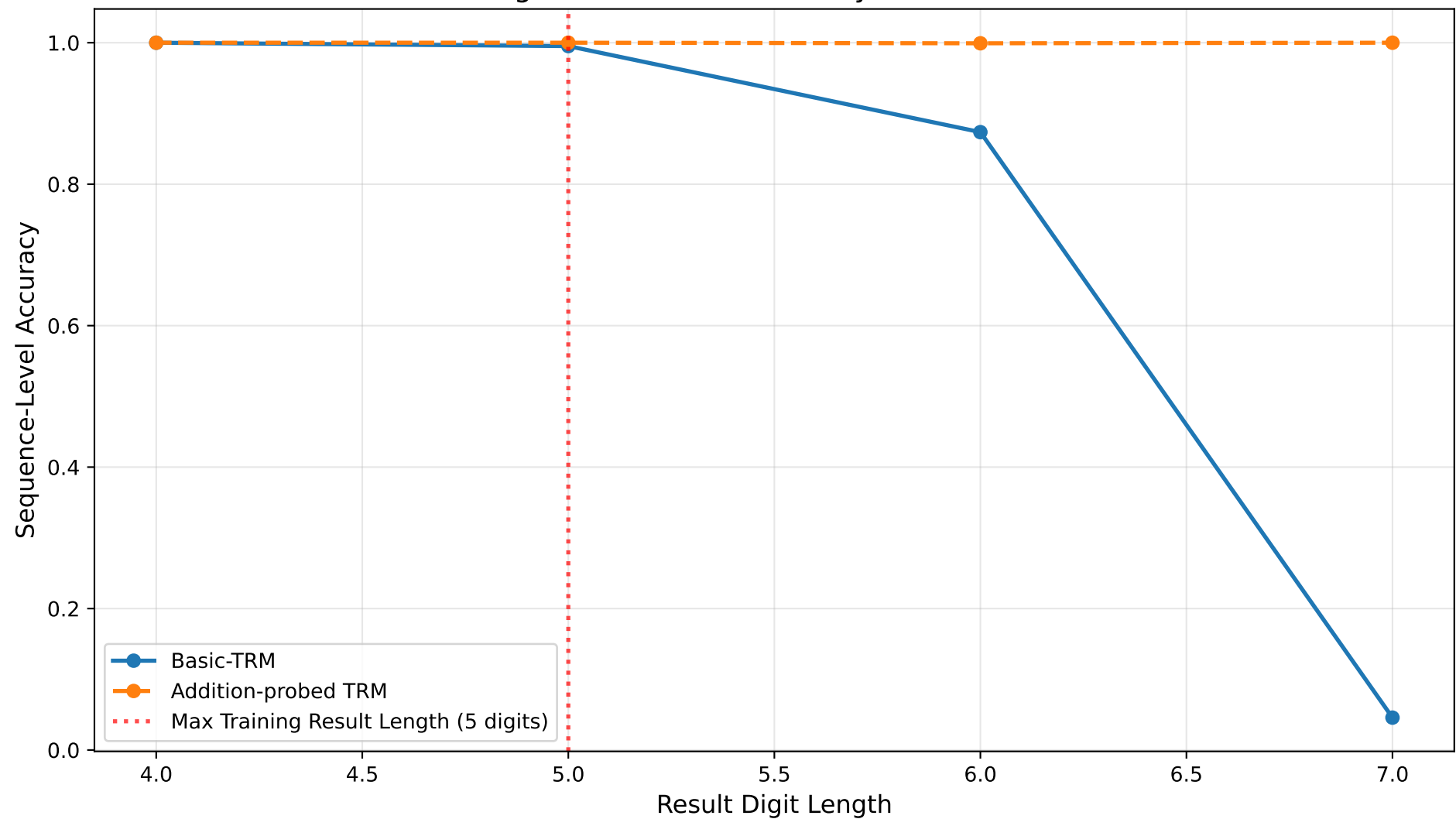
Length Generalization Analysis for Addition
