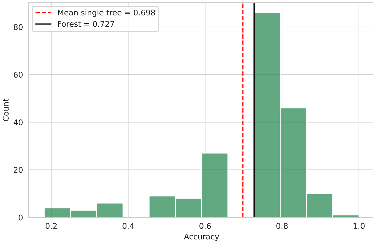
Individual Trees vs the Full Forest (Test Accuracy)
