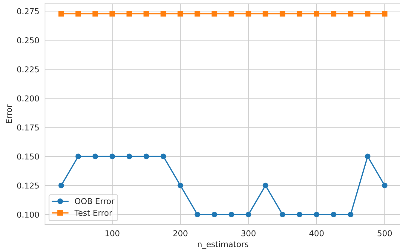
Error vs Number of Trees
