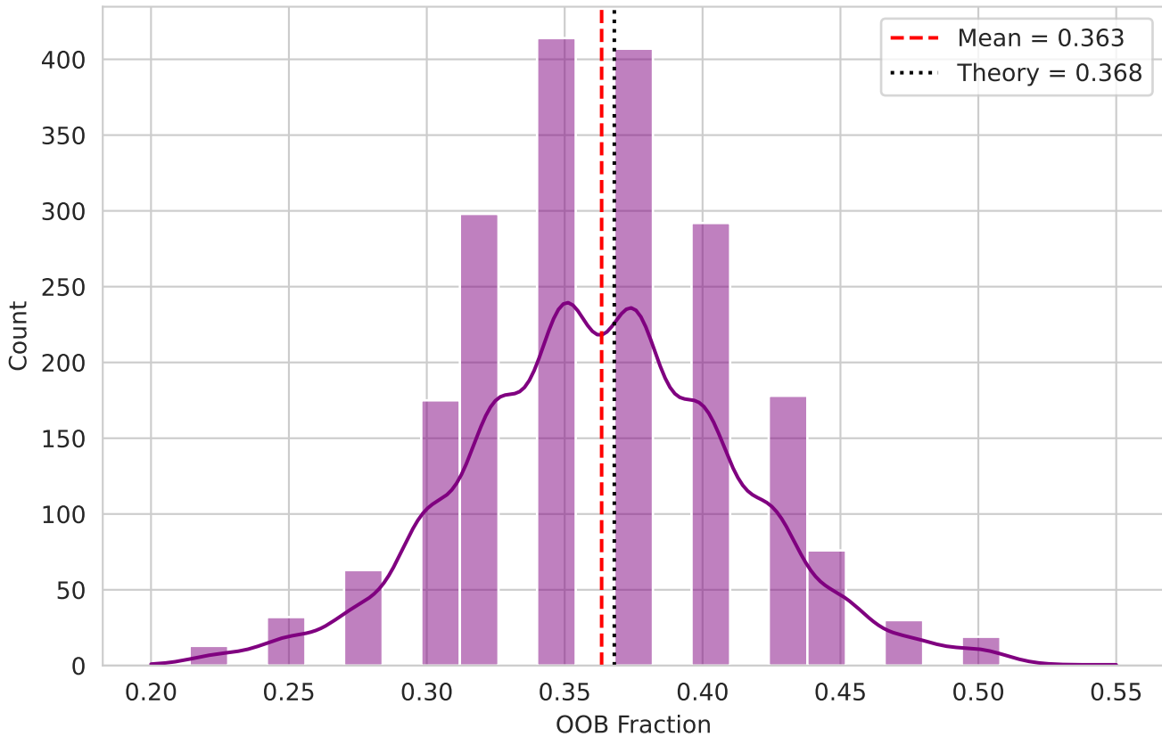
Out-of-Bag Fraction Across 2000 Bootstrap Samples
