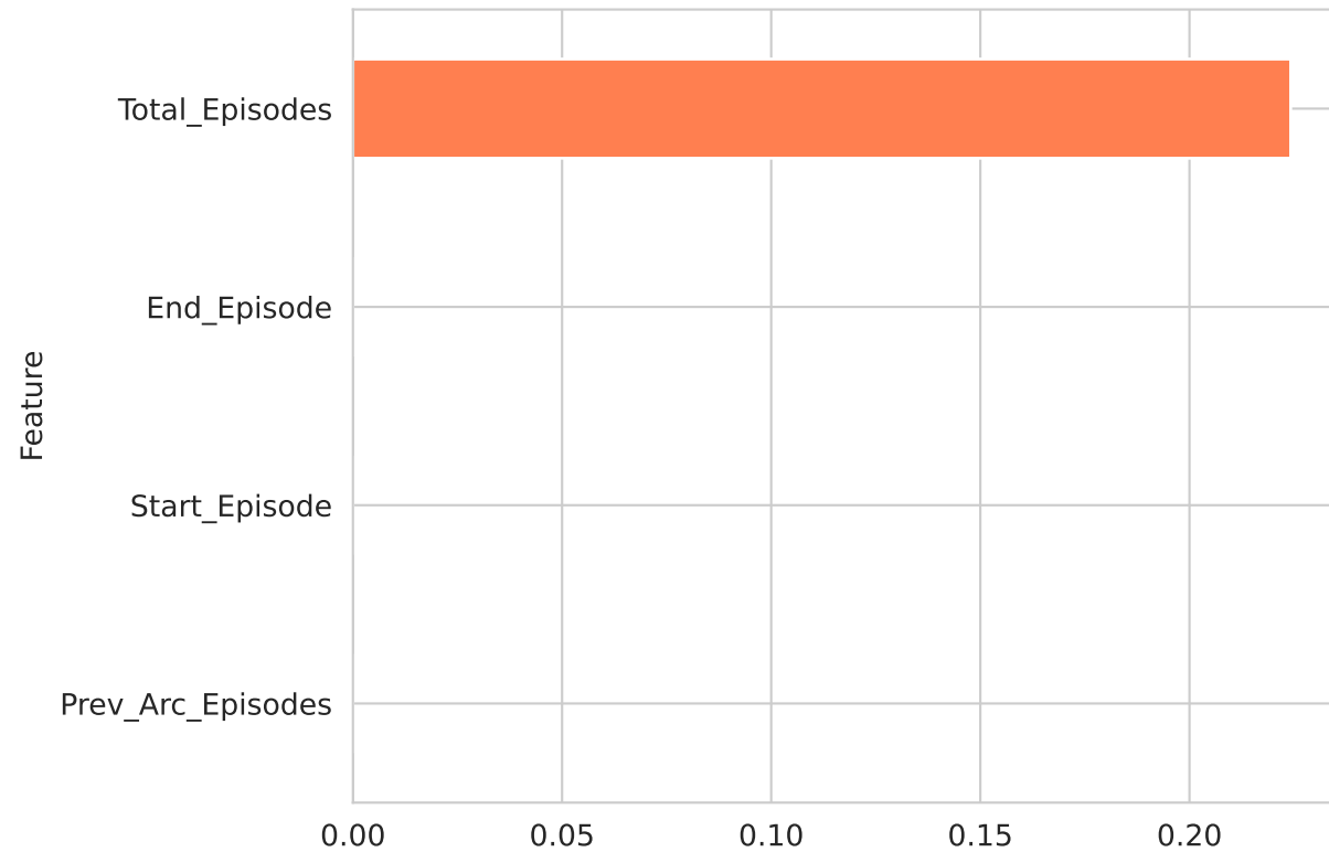
Permutation Importance (Test Set)
