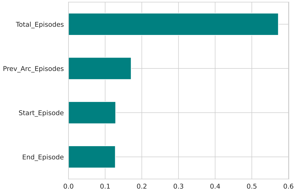
Random Forest Impurity Importance
