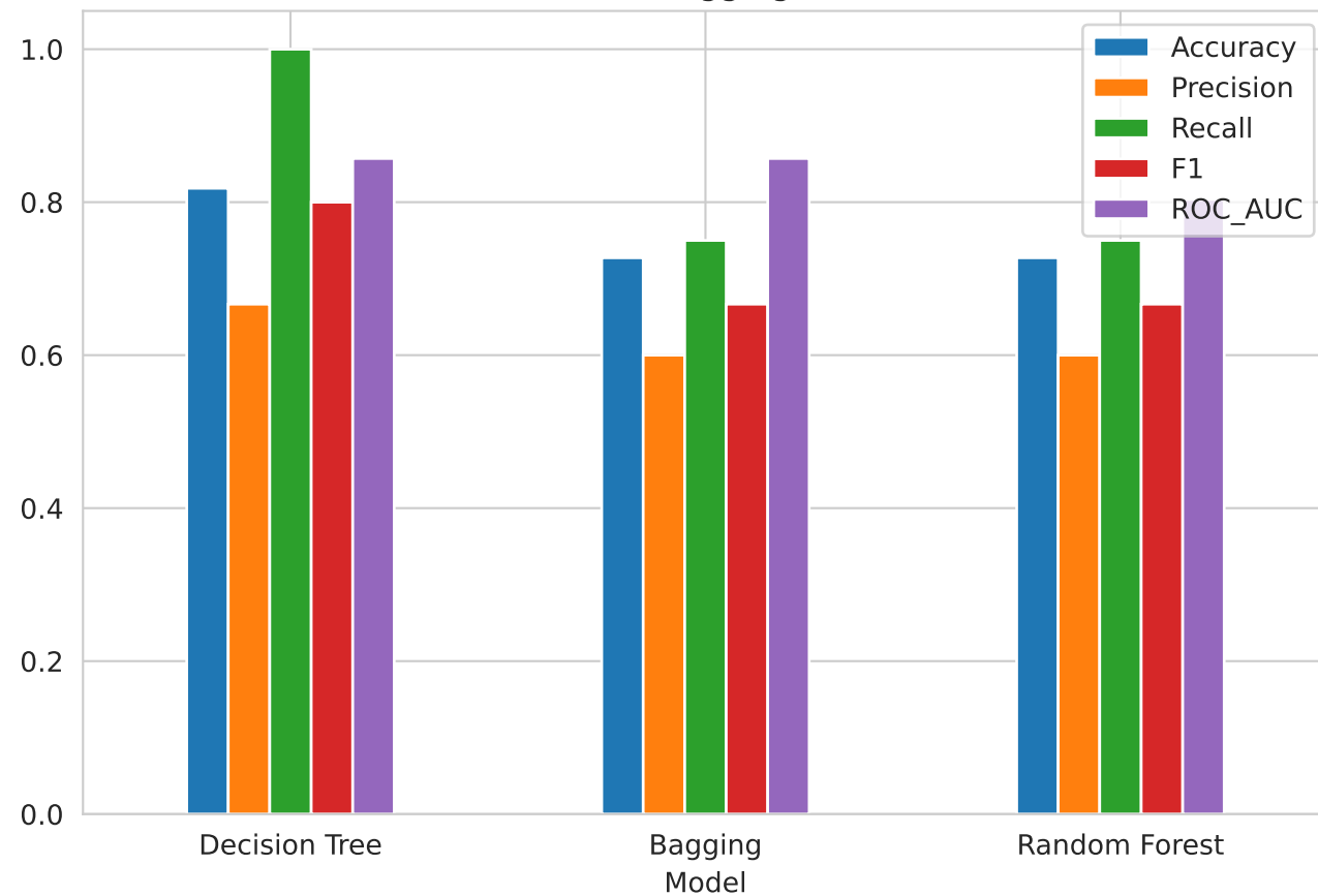
Test Metrics: Tree vs Bagging vs Random Forest
