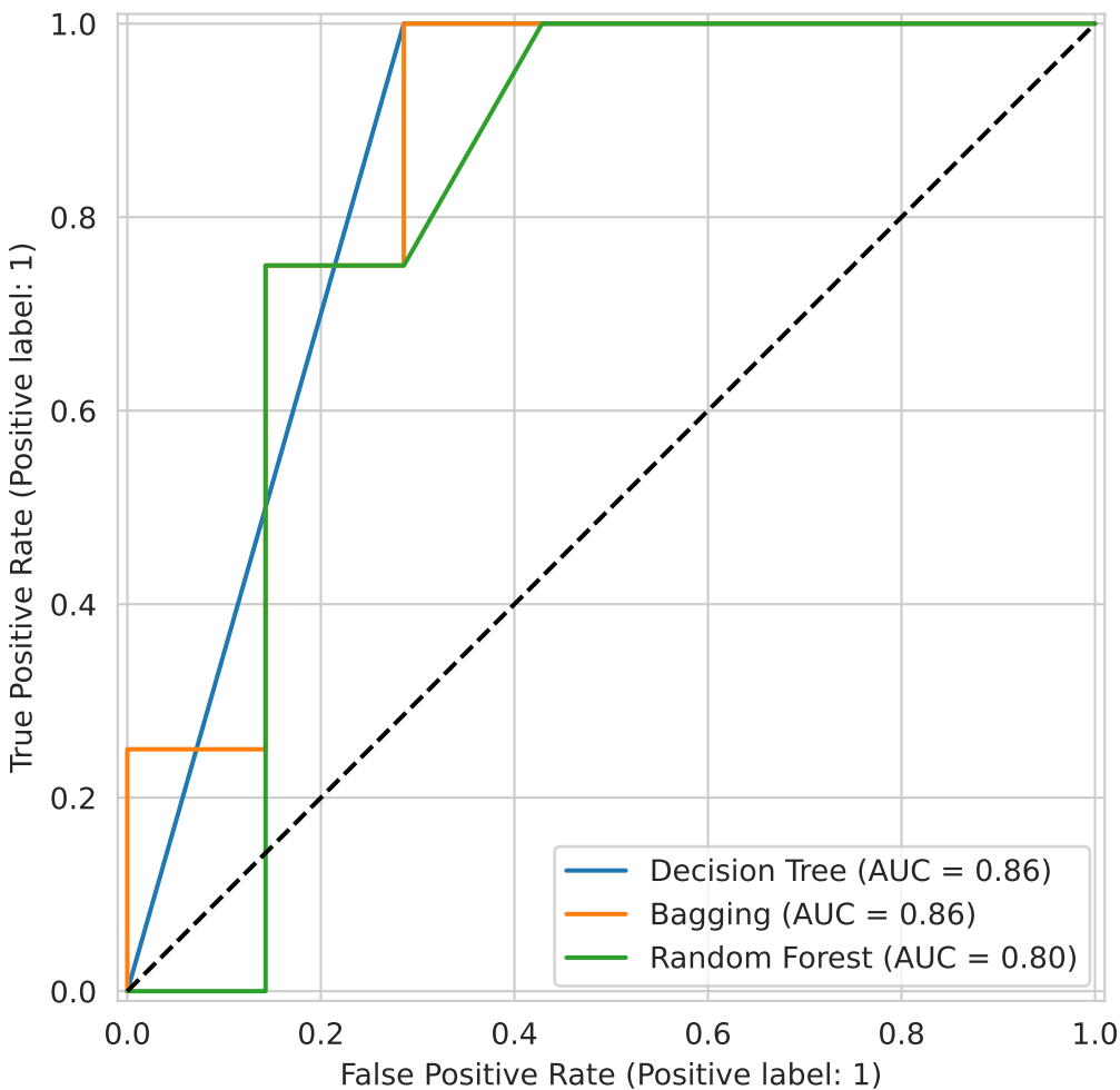
ROC Curves
