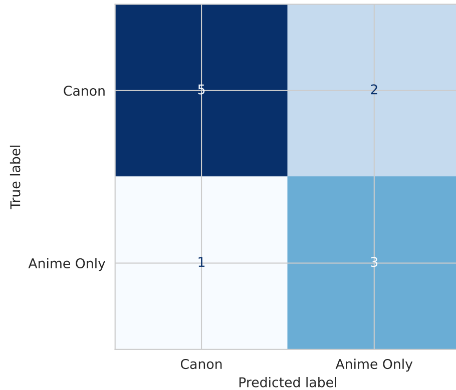
Bagging
