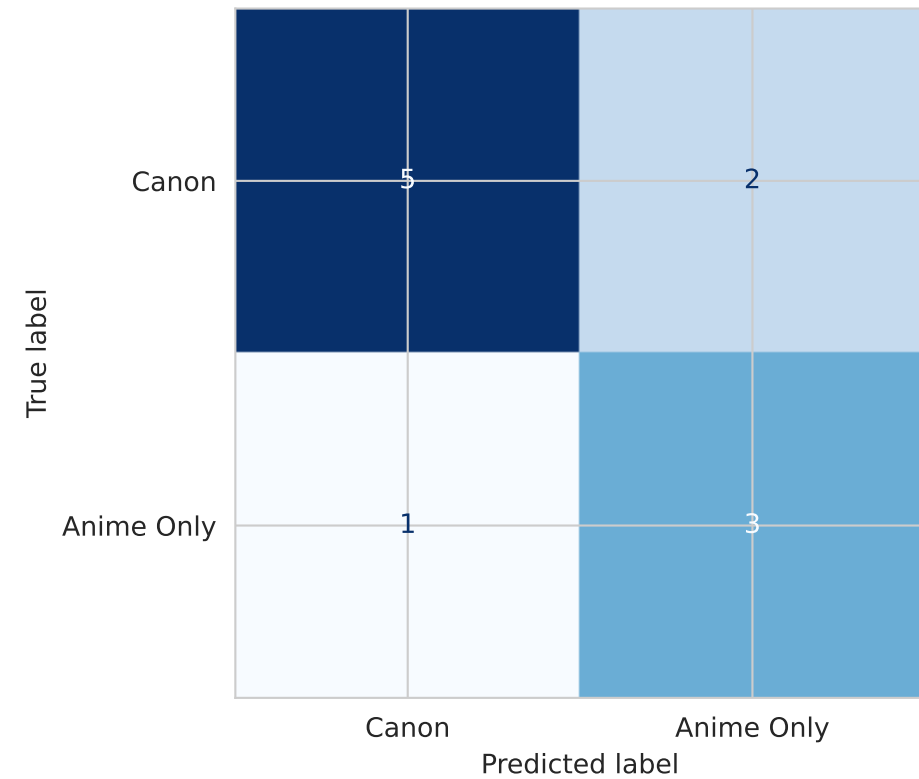
Random Forest
