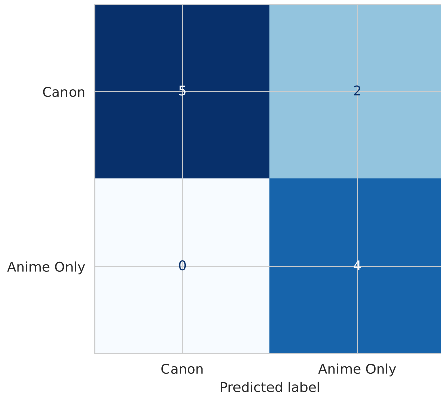
Decision Tree
