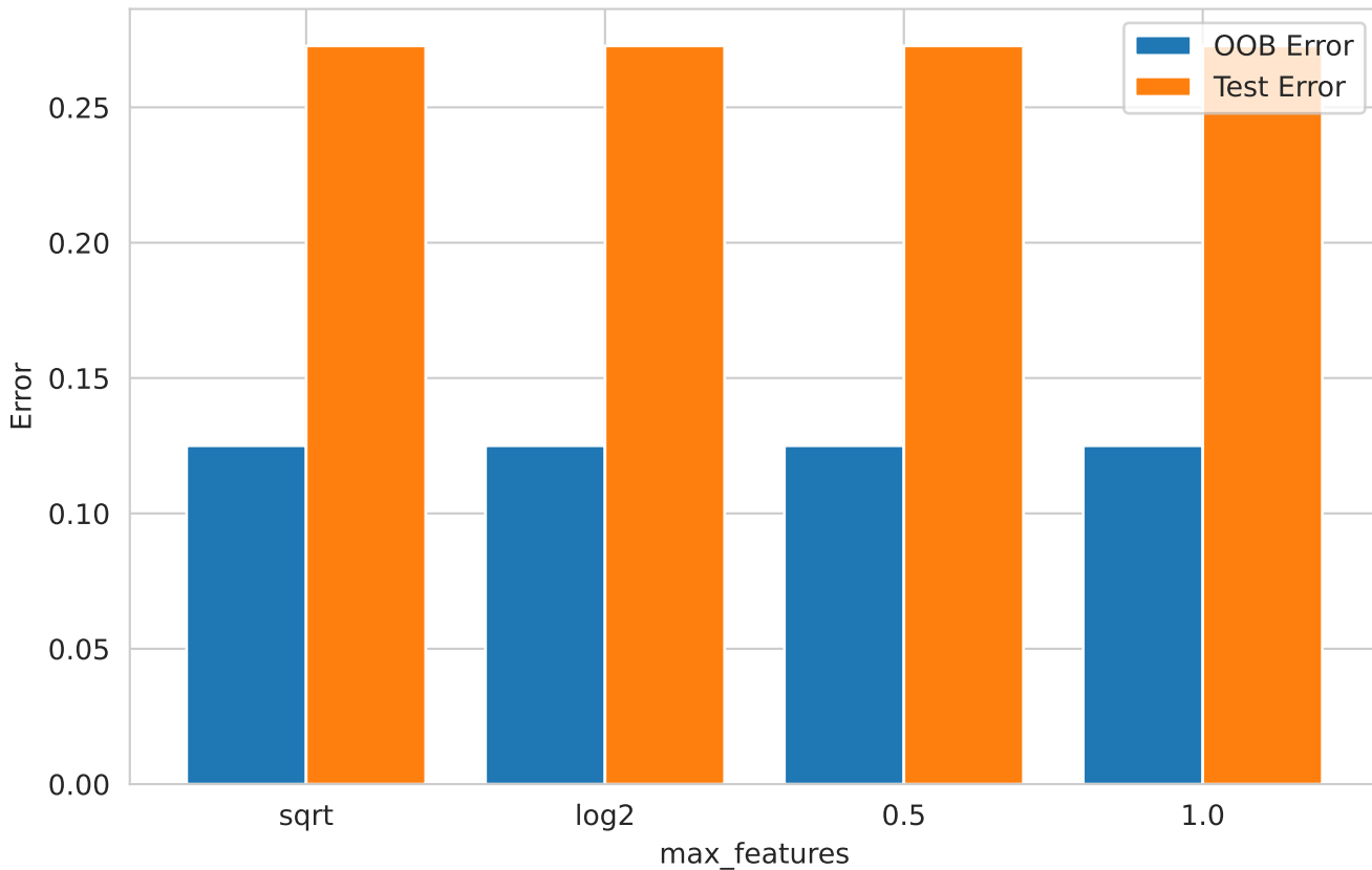
Feature Subsampling: OOB Error vs Test Error
