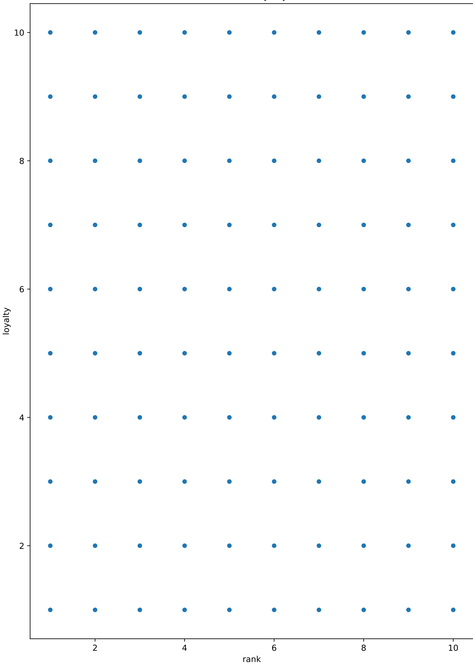
rank vs loyalty
