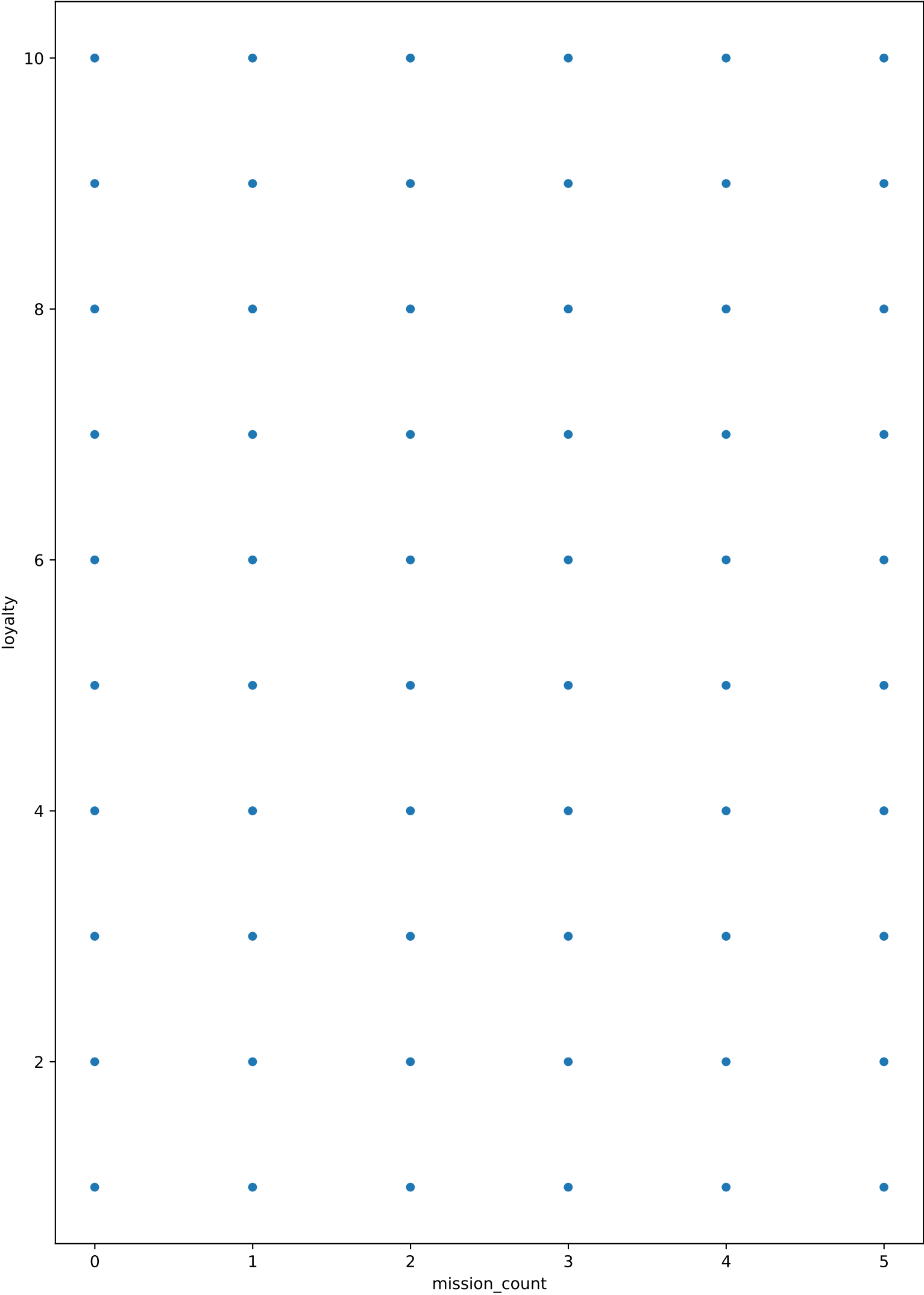
mission_count vs loyalty
