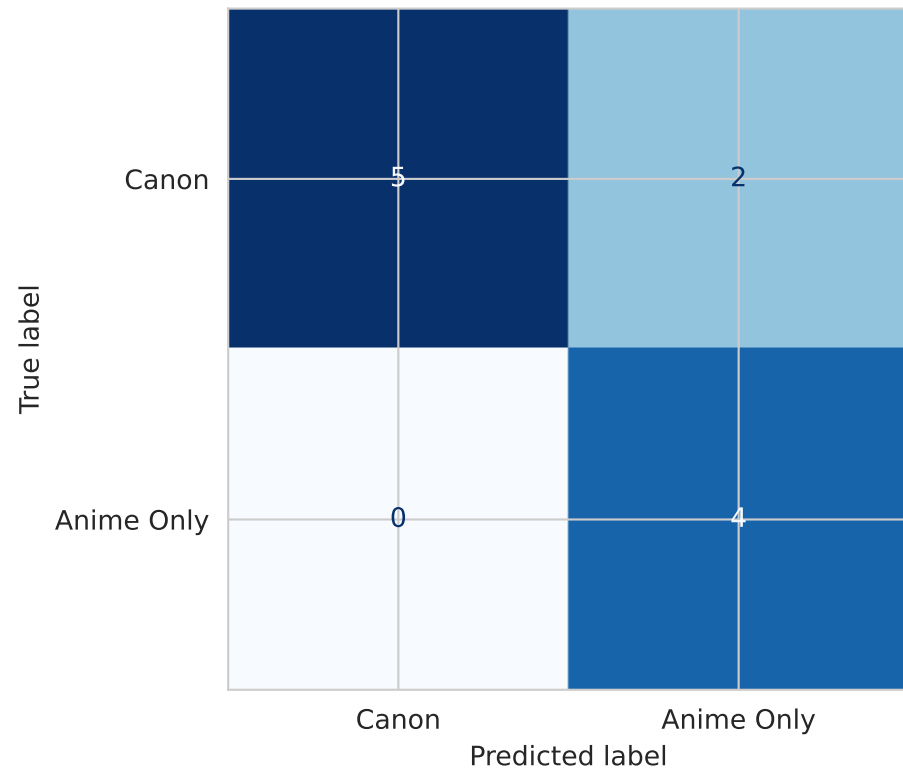
Confusion Matrix: Entropy
