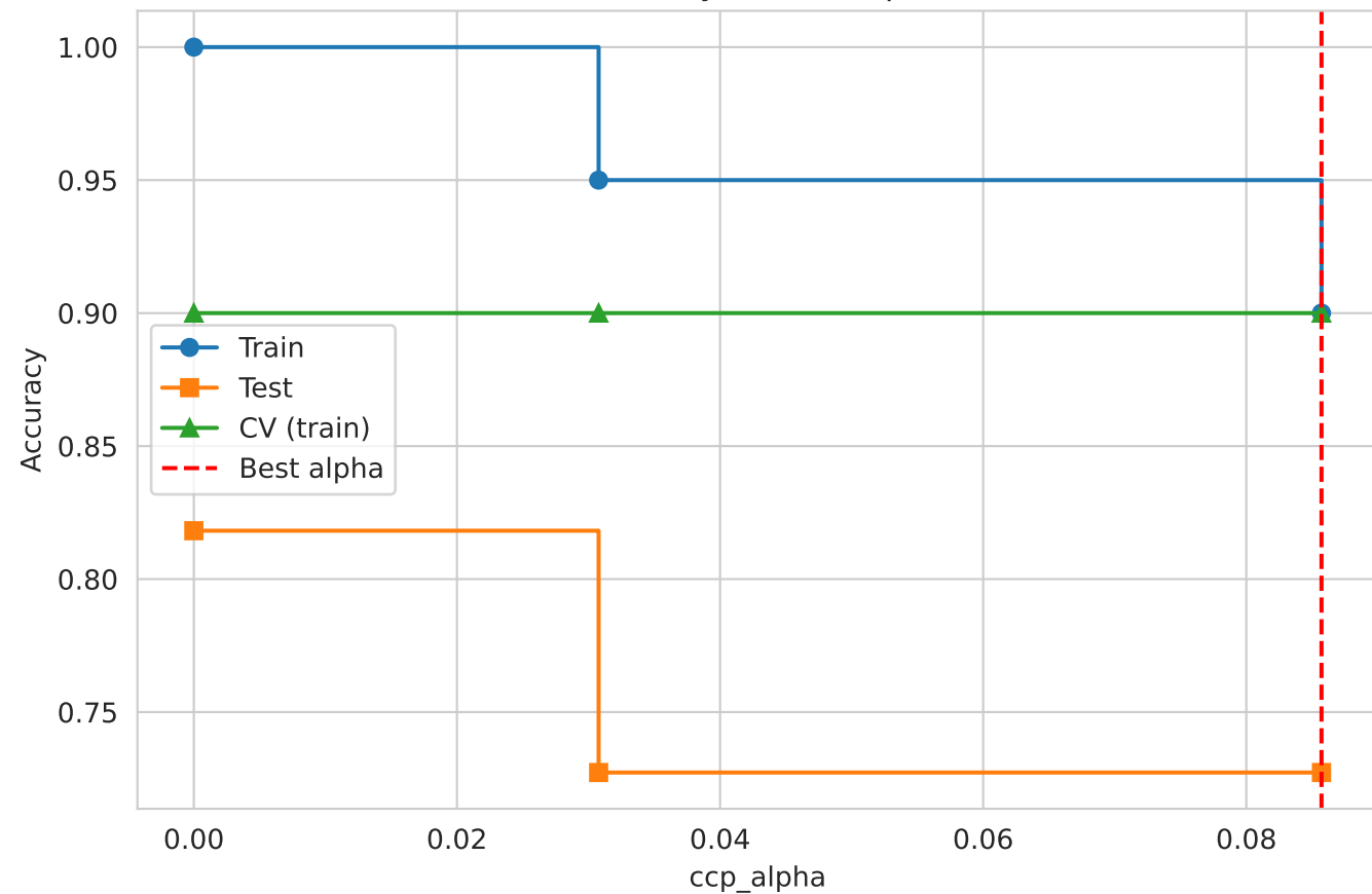
Accuracy vs CCP Alpha
