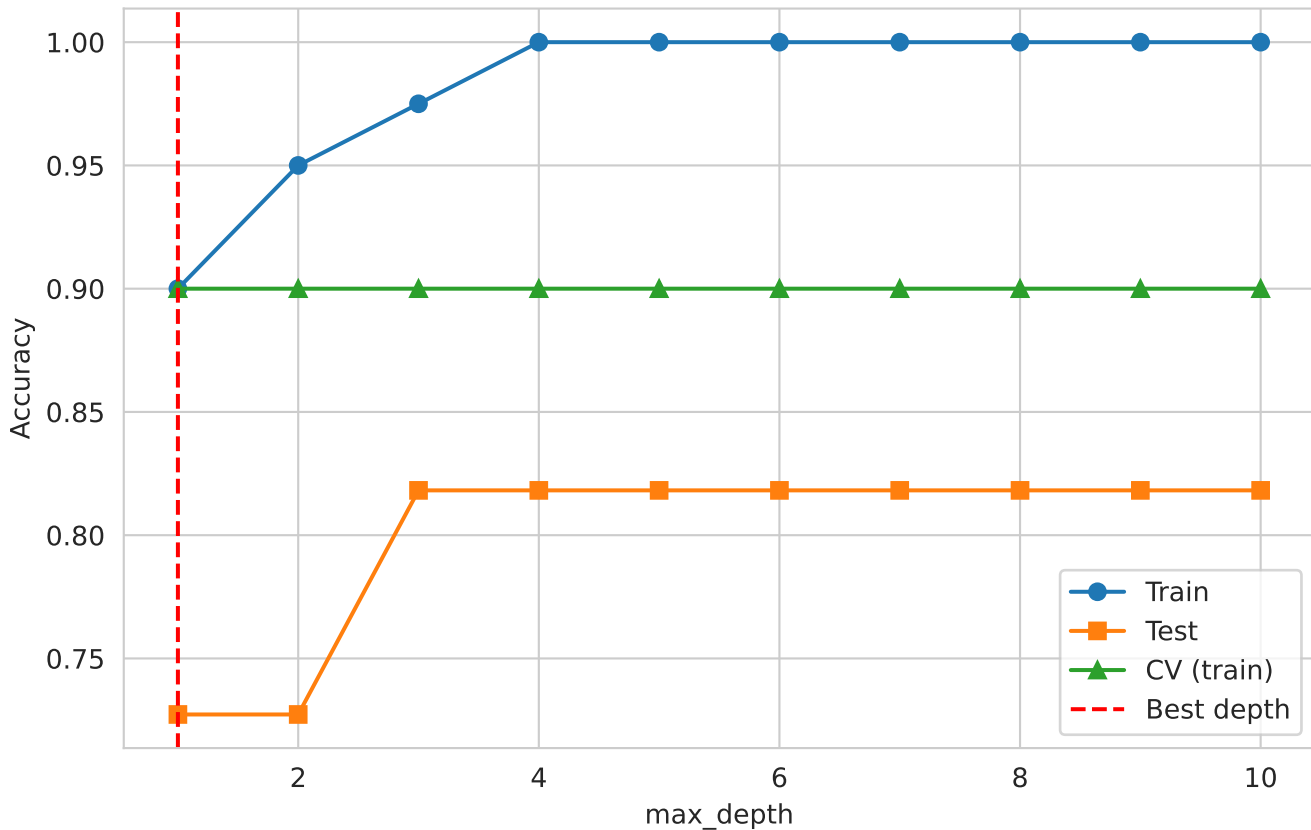
Depth Sweep: Train vs Test vs CV Accuracy
