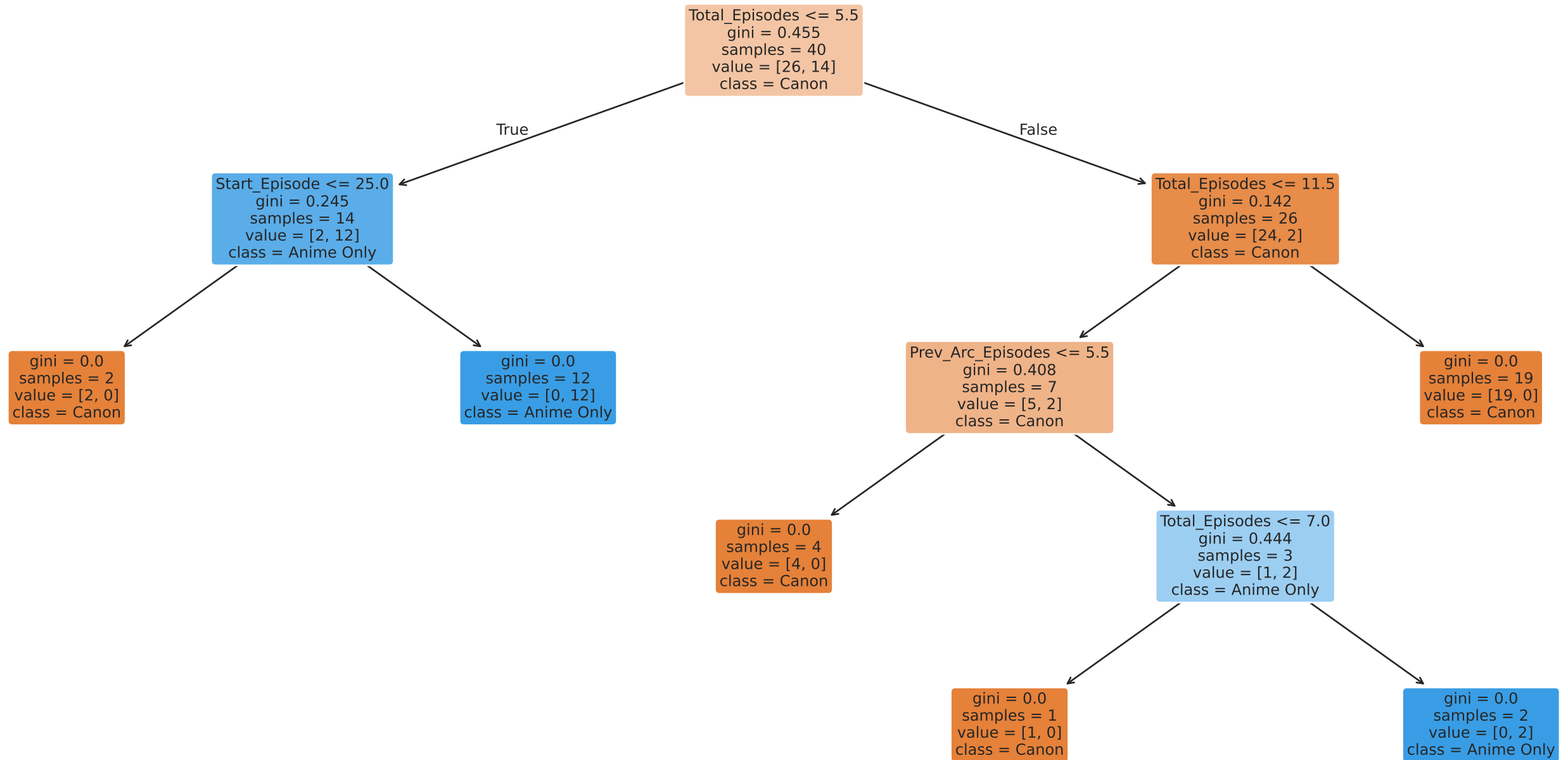
Decision Tree Structure: Gini
