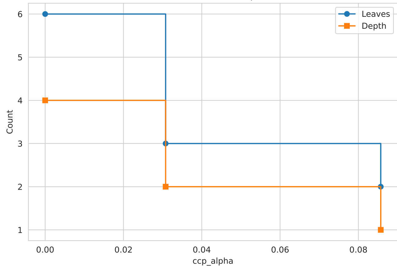
Tree Size vs CCP Alpha
