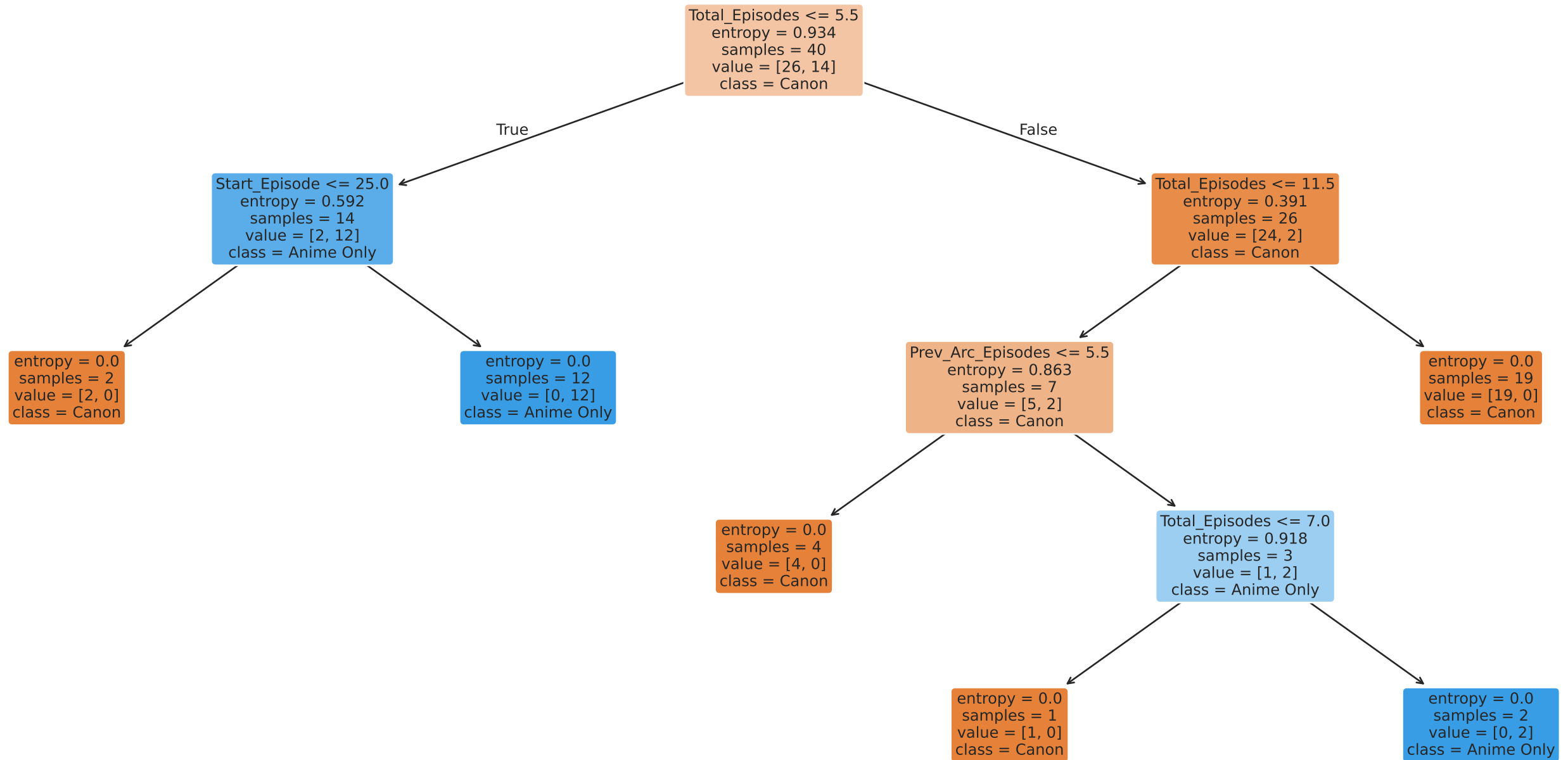
Decision Tree Structure: Entropy
