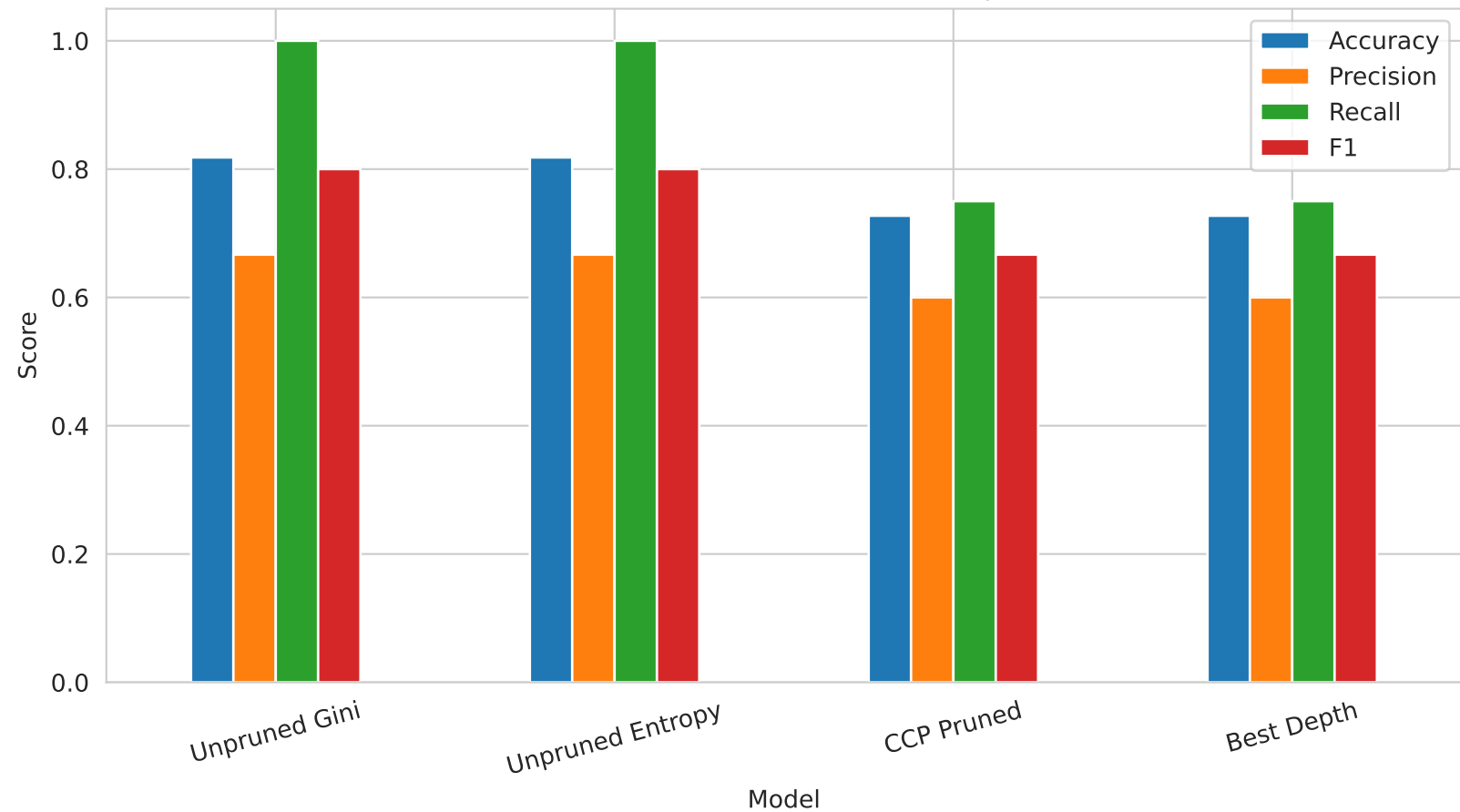
Decision Tree Variants: Metric Comparison
