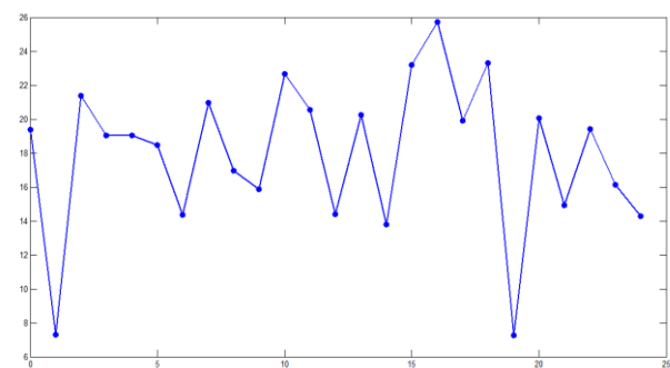
Fig 2. Average turbidity
