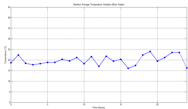
Fig 1. Average temperature
