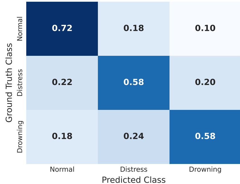
EXP-A: Spatial YOLO (Baseline)
