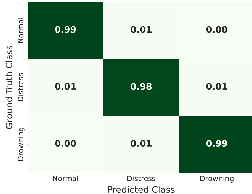
EXP-C: Proposed Bi-LSTM
