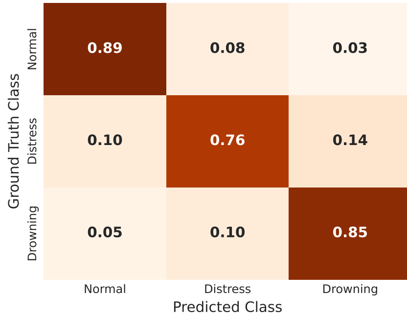
EXP-B: YOLO + Rule Filter
