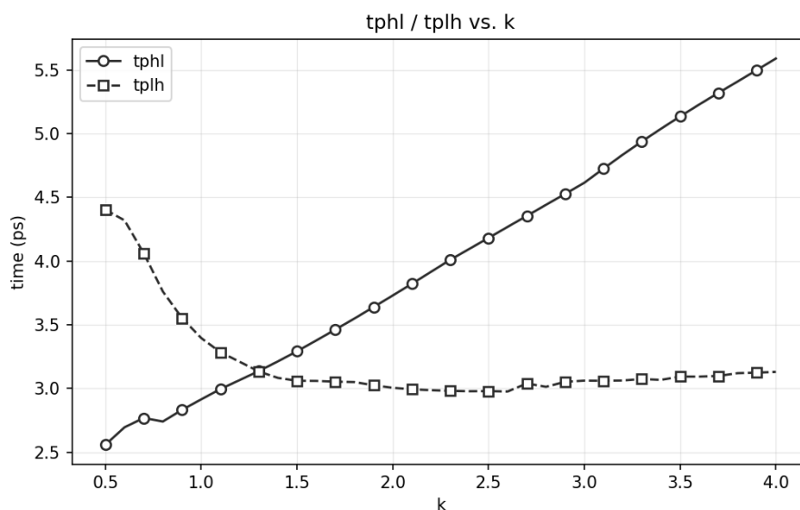
Figure 1: tpHL and tpLH vs K, X=10p
