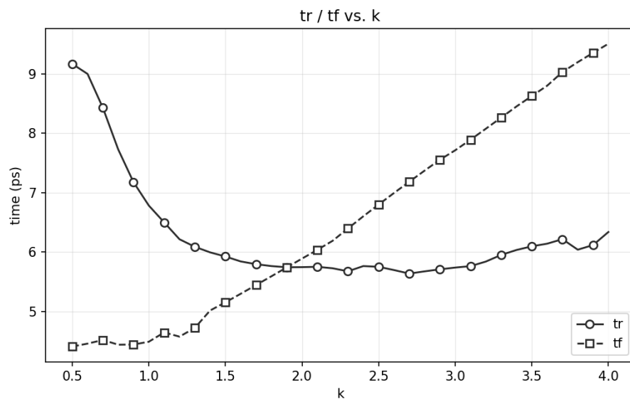
Figure 4: tr and tf vs K, X=5.65p
