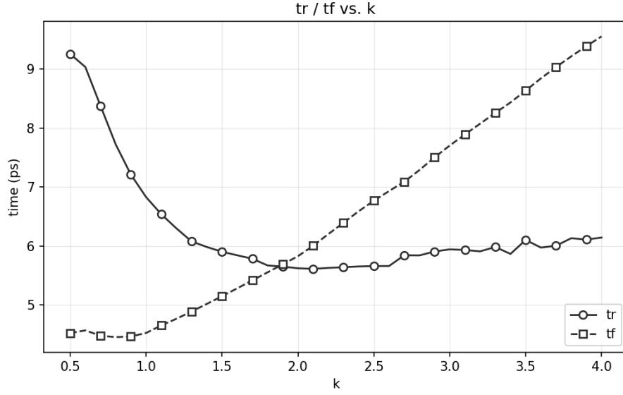
Figure 2: tr and tf vs K, X=10p
