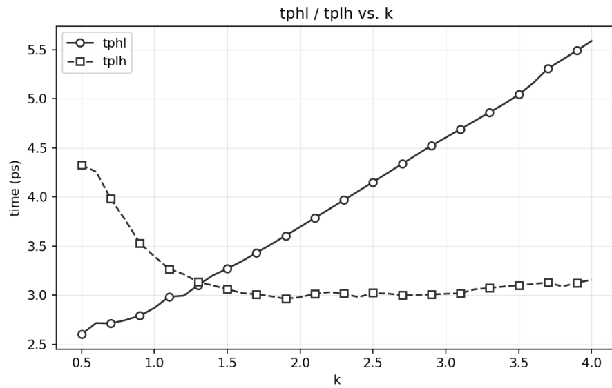
Figure 3: tpHL and tpLH vs K, X=5.65p
