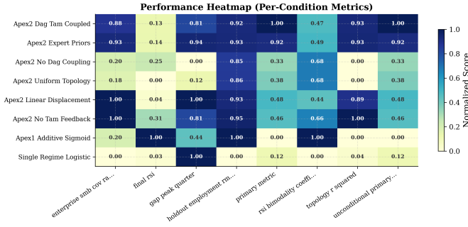
Fig. 10. Metric heatmap used to inspect variation across model variants and reported outcomes.
