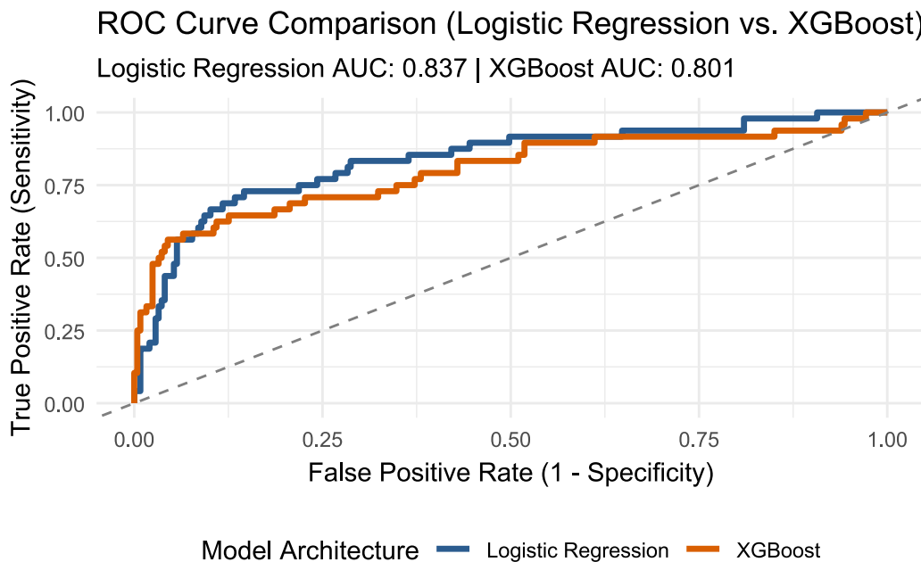
Figure 4: Combined ROC Curves for Attrition Prediction Models
