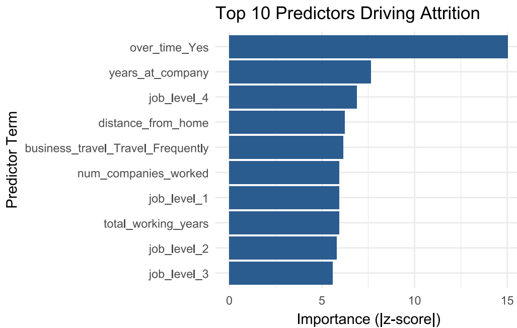
Figure 3: Top 10 Feature Importance Scores for Attrition Prediction
