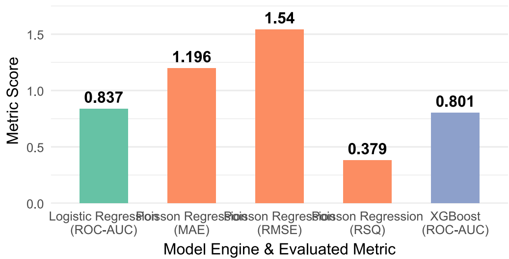
Figure 5: Comparative Overview of Model Metrics Across Prediction Engines
