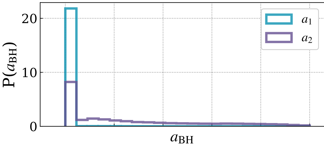
K26 with Bavera et al. (2021) Fit
