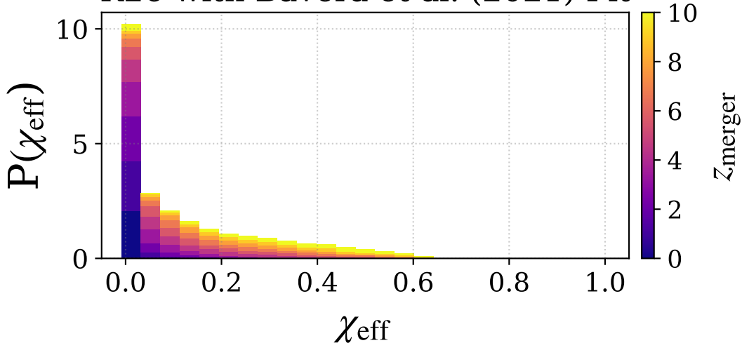
K26 with Bavera et al. (2021) Fit
