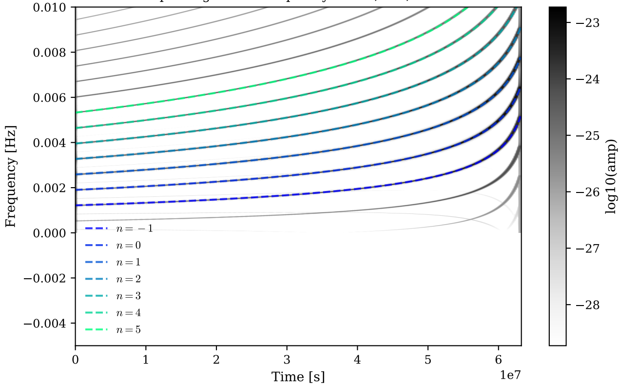
Spectrogram vs. frequency tracks, l=2 , m=2
