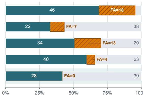
FinanceBench ( n = 67 )
