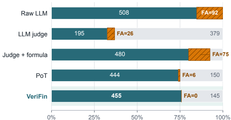
XBRLBench ( n = 600 )
