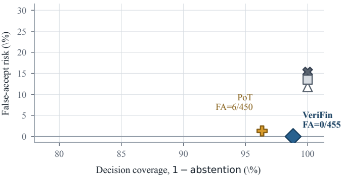
XBRLBench ( n = 600 )
