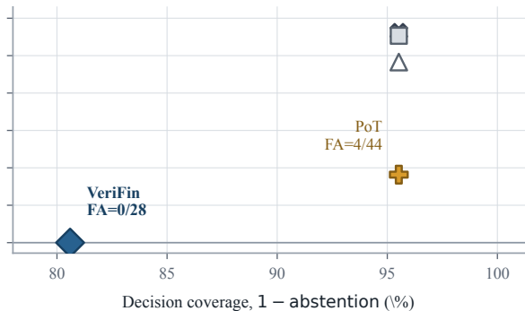
FinanceBench ( n = 67 )
