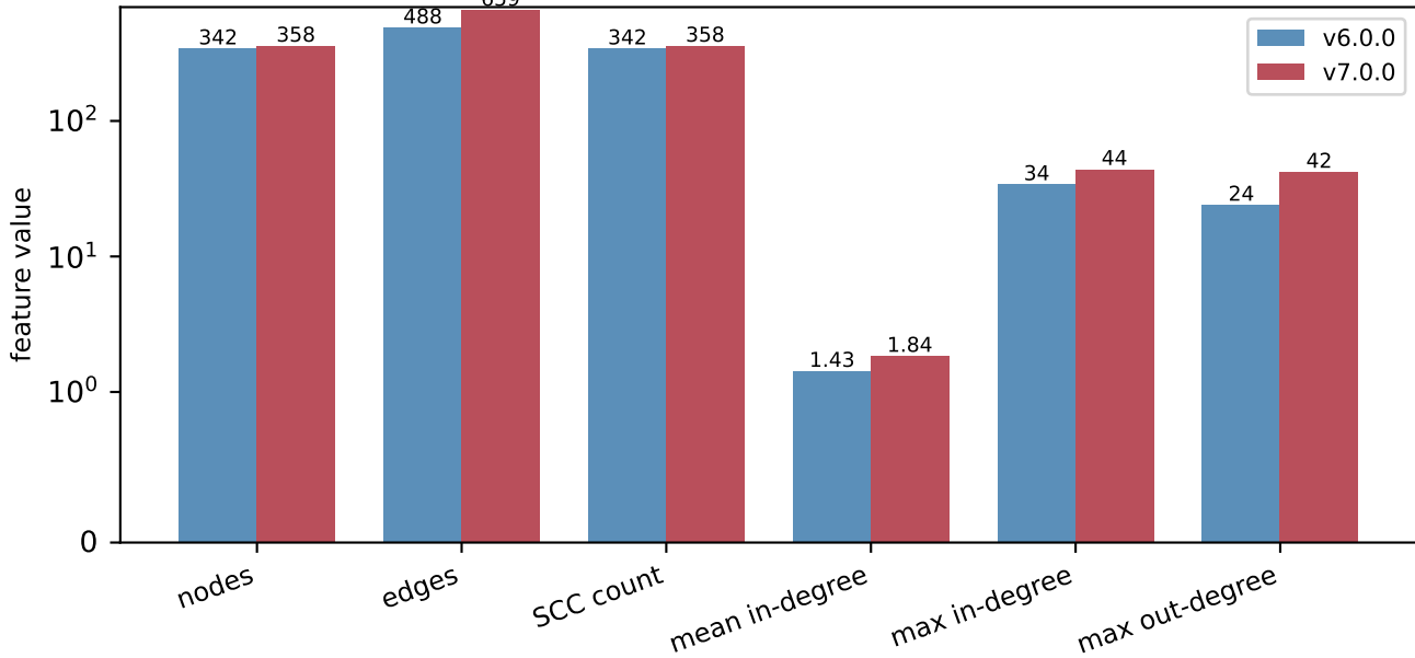
C06a call-graph topology features, chardet v6 vs v7
