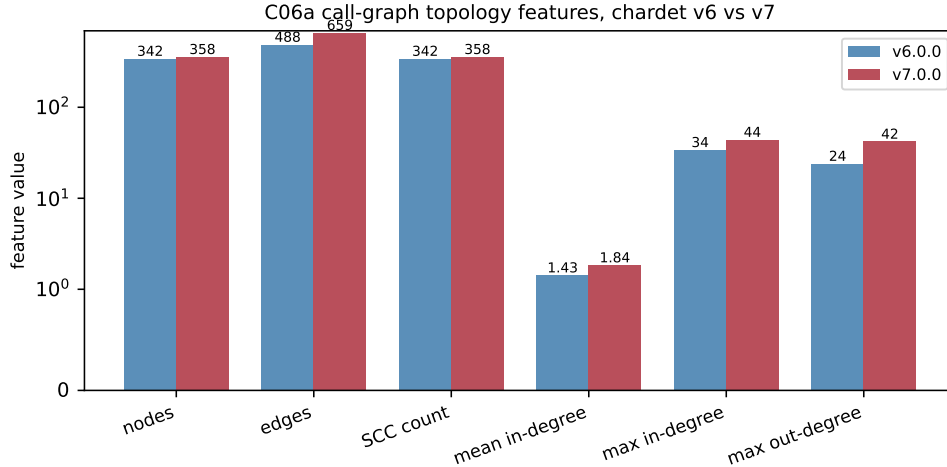
Figure 2: C06a call-graph topology features for chardet v6 and v7. v7 is larger on every feature (more nodes, more edges, larger maximum in-degree) but the relative differences are small enough to yield a mean similarity of 0.881.
