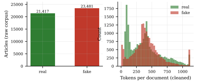
Fig. 9. Raw class counts (left) and token-length distributions after normalisation, clipped at the 98th percentile for legibility (right).
