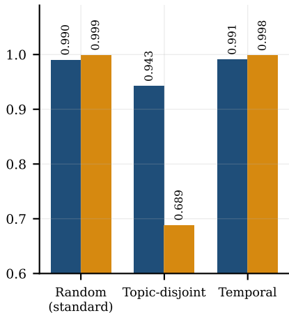
F_1 (prior-matched)
