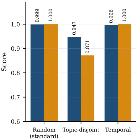
Average precision
