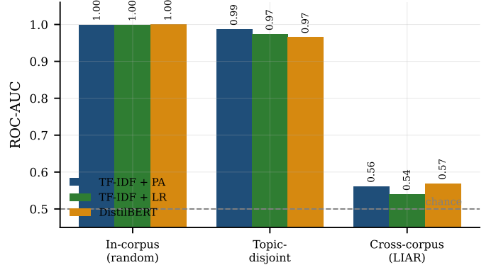
Fig. 10. ROC-AUC of each model across three evaluation regimes: in-corpus random split, in-corpus topic-disjoint split, and cross-corpus transfer to LIAR. Ranking quality survives topic shift within ISOT but collapses to near-chance on an independently constructed corpus. The dashed line marks chance (0.5).
