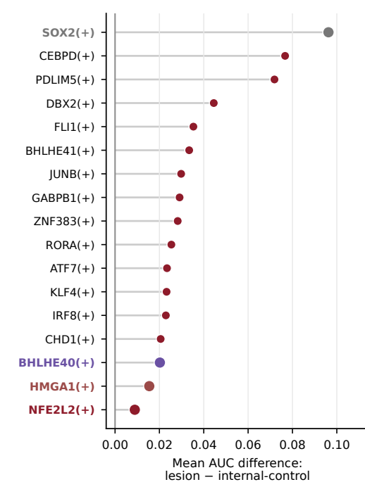
Top lesion-associated regulons
