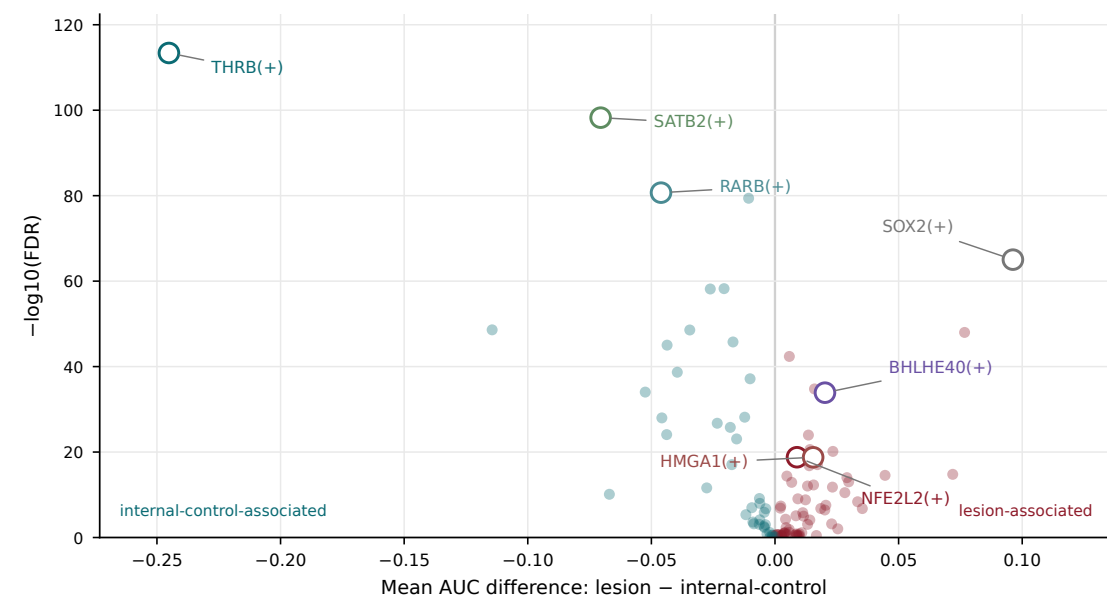
All-regulon differential summary
