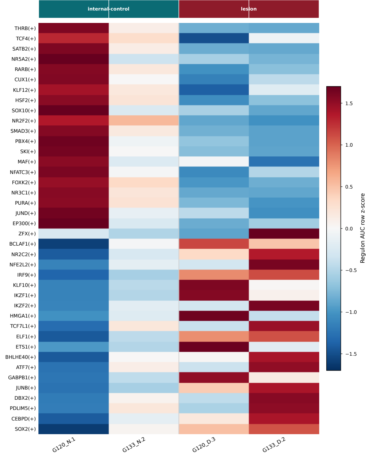
Top 40 differential regulon heatmap
