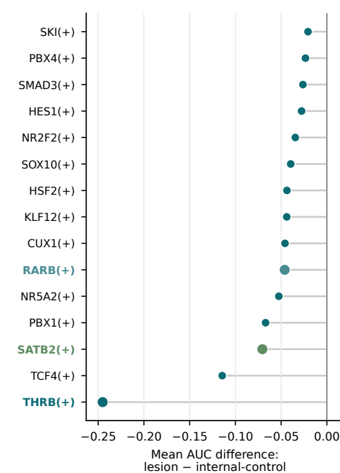
Top internal-control-associated regulons
