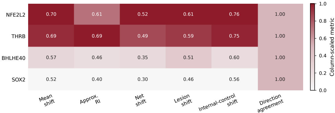
Round 1 CellOracle perturbation metric heatmap
