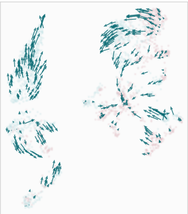
THRB representative in silico KO
