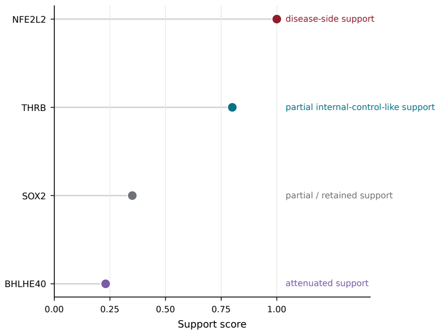
GSE140393 ranked single-group support score
