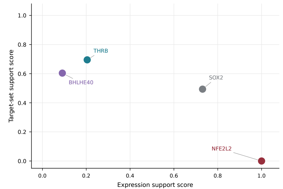
GSE190452 cross-syndrome expression and target-set support
