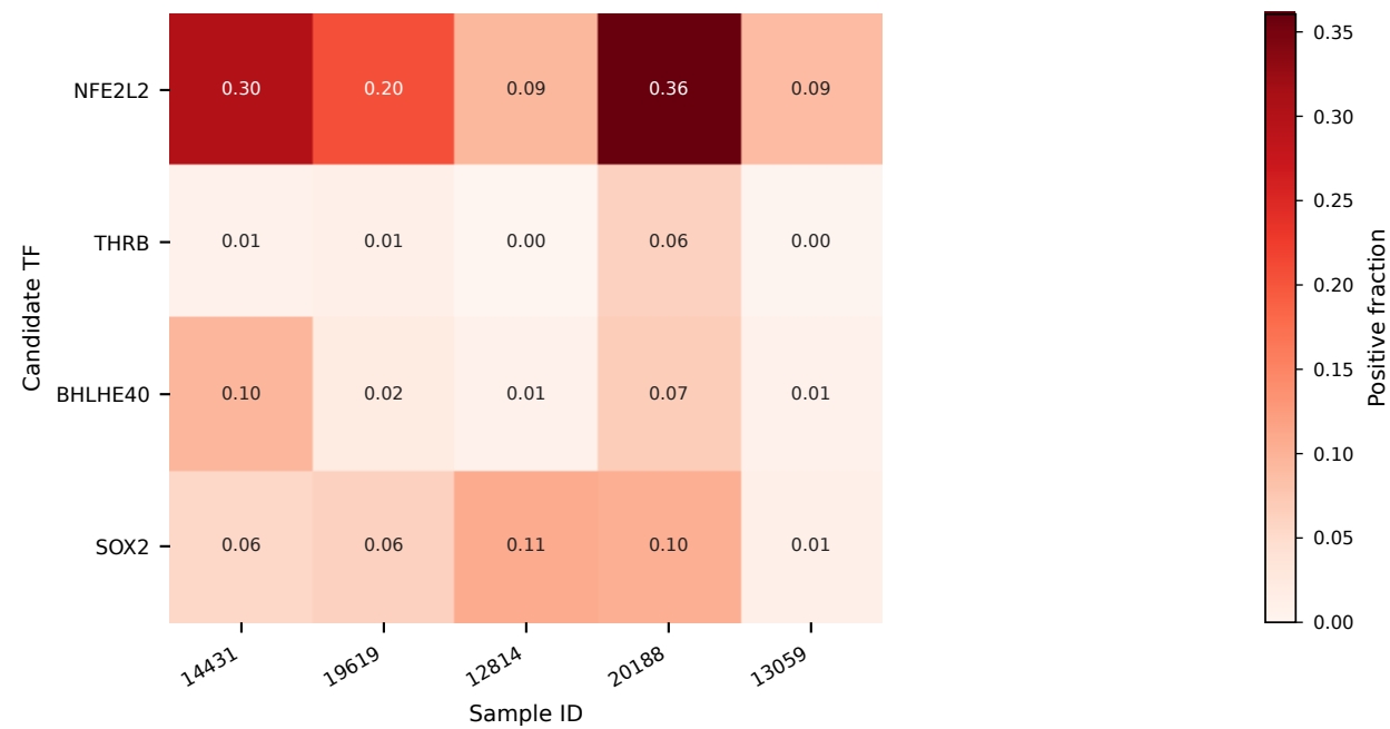
GSE140393 single-group expression support
