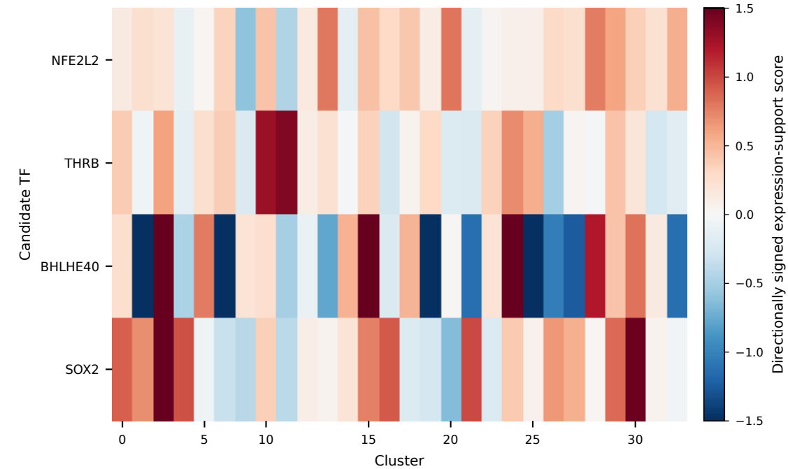
GSE190452 cluster-level expression-support pattern
