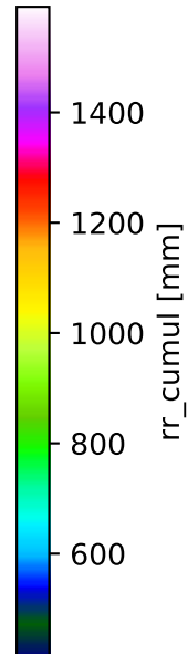
Total precipitation between 20210801 and 20220701
