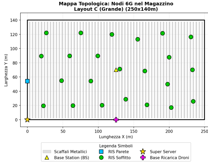
Figura 10: Layout C VNA (250x140m, 24 RIS)
