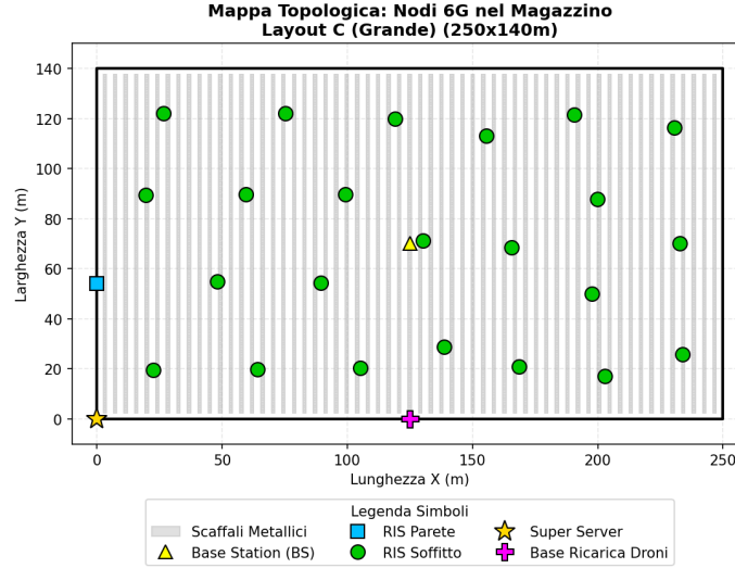
Figura 11: Layout C VNA (250x140m, 24 RIS)
