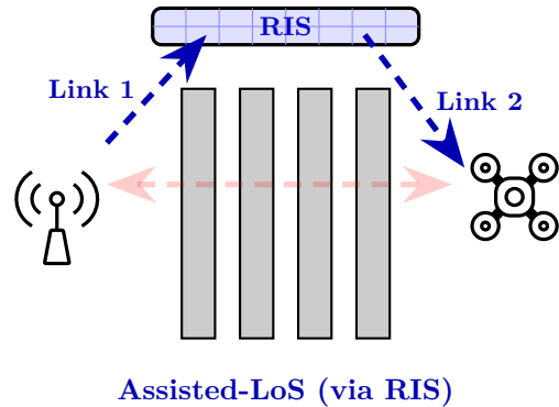
Scenario Assisted-LoS
