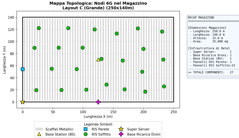
Figura 6: Layout C VNA (250x140m, 24 RIS)
