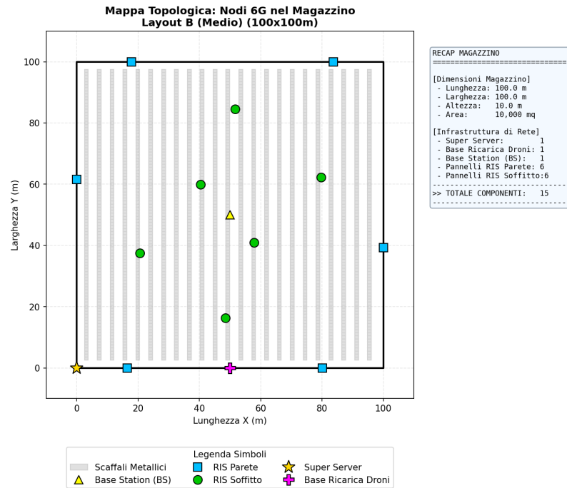
Figura 5: Layout B (100x100m, 12 RIS)
