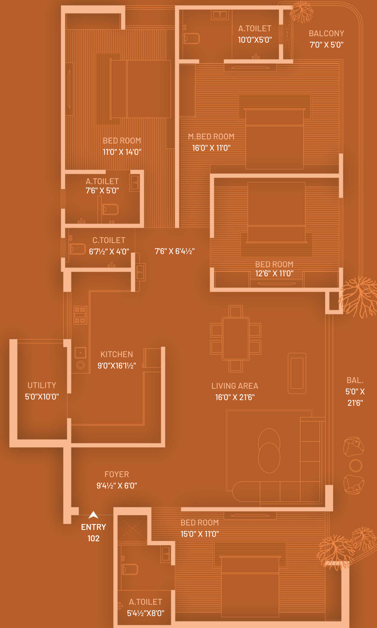
4 - BHK TYPICAL UNIT PLAN BUILDING - B
