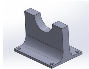
Detecting contours
