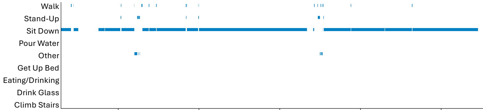
GT Activity
