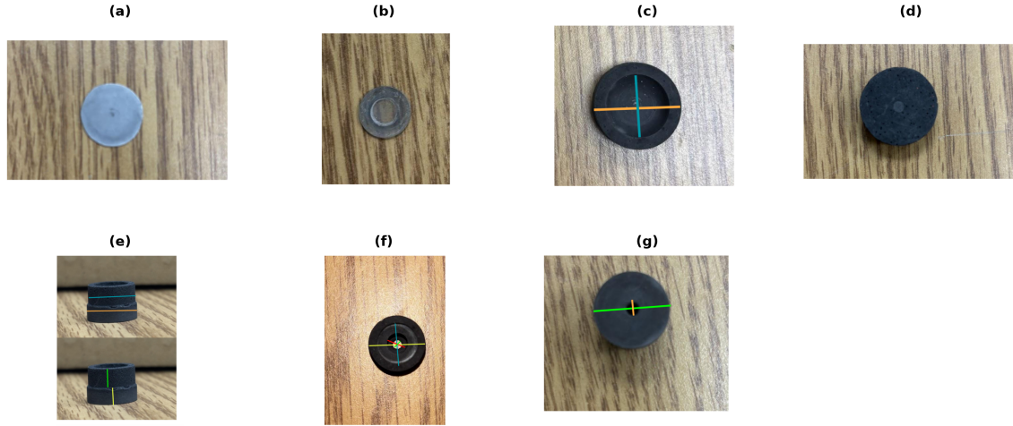
Figure S1: Measured dimensions of each part of the graphite crucible/susceptor assembly; each dimension is keyed to the colour of the measurement line drawn on the photograph. (a) Alumina spacer disc, 14 mm dia. (b) Sapphire pyrometer window, 9.5 mm dia., 0.5 mm thick. (c) Crucible body, top: machined sample cavity 14.55 mm ID (teal) and 20.30 mm OD (orange); the cup is 6.5 mm tall with a 2 mm base. (d) Crucible body, bottom face, 20.30 mm dia. (e) Crucible lid, oblique, with the stepped plug that seats into the cavity: 13.70 mm upper-step diameter (teal) and 14.55 mm lower-shoulder diameter (orange); the upper step is 6 mm tall (green) and the lower shoulder 4 mm tall (yellow). (f) Crucible lid, top: 13.70 mm outermost diameter (yellow), 9.75 mm second step (teal), 5 mm third step (red), and the 3.5 mm central pyrometer-sighting bore (green). (g) Crucible lid, bottom: 14.55 mm seating face (green) and the 3.5 mm through-bore (orange). Fully assembled the crucible stands 13 mm tall.
