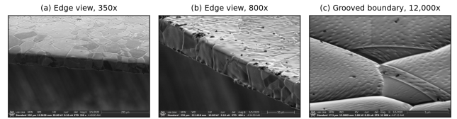
FIG. 8. Grain-boundary thermal grooving on a Ni4N5 specimen after a 1200^{\circ}\text{C} / 12 h anneal, imaged edge-on in the as-annealed condition after only an ultrasonic ethanol clean. (a) Edge view at 350\times ( 200\text{ }\mu\text{m} scale bar). Several grain boundaries traverse the full sheet thickness. (b) Edge and top surface at 800\times ( 50\text{ }\mu\text{m} scale bar). The grooves outline the surface grain structure. (c) A single grooved boundary at 12,000\times ( 5\text{ }\mu\text{m} scale bar). The deep trench develops as grain-boundary energy equilibrates against surface energy at the soak temperature.
