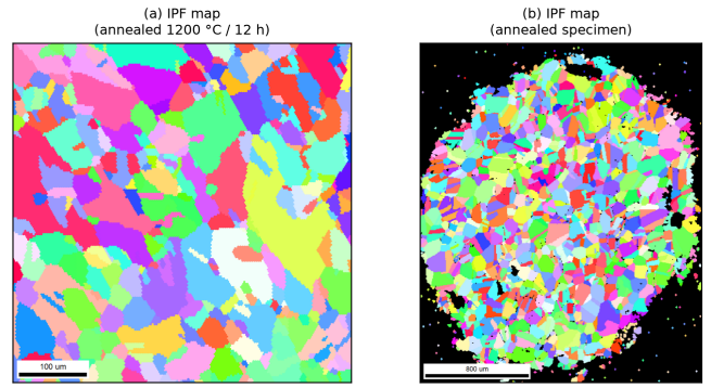
FIG. 7. EBSD inverse-pole-figure (IPF) orientation maps of two furnace-annealed Ni4N5 specimens, rendered from the recorded EBSD scans. (a) A specimen annealed at 1200^{\circ}\text{C} for 12 h ( 100\text{ }\mu\text{m} scale bar). (b) A second annealed specimen ( 800\text{ }\mu\text{m} scale bar). The maps resolve hundreds of grains for grain-size and texture analysis.
