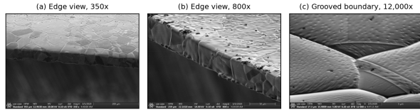
FIG. 5. Grain-boundary thermal grooving on a Ni (4N5) specimen after a 1200 ^{\circ}\text{C} / 12 h anneal, imaged edge-on in the as-annealed condition after only an ultrasonic ethanol clean. (a) Edge view at 350 \times (200 \mu\text{m} scale bar). Several grain boundaries traverse the full sheet thickness. (b) Edge and top surface at 800 \times (50 \mu\text{m} scale bar). The grooves outline the surface grain structure. (c) A single grooved boundary at 12,000 \times (5 \mu\text{m} scale bar). The deep trench develops as grain-boundary energy equilibrates against surface energy at the soak temperature.
