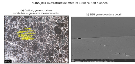
FIG. 6. Microstructure of a Ni (4N5) specimen after a 1300 ^{\circ}\text{C} / 20 h anneal under a constant 20 SCCM argon flow. (a) Optical grain map with in-image grain-size measurements (200 \mu\text{m} scale bar); (b) high-magnification SEM grain-boundary detail.
