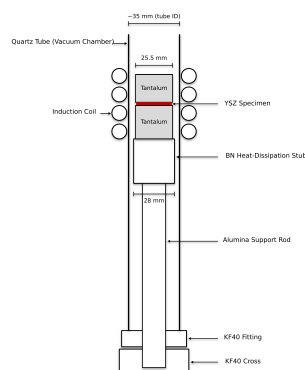
FIG. 8. Sample-stack configuration for the high-temperature ceramic anneals. The YSZ specimen is sandwiched between two 25.5 mm tantalum susceptor blocks inside the quartz tube. The blocks rest on a boron nitride heat-dissipation stub, which sits on the alumina support rod that raises the sample stack to coil height. The coil, vacuum, pyrometer, and control paths are unchanged from the metal configuration.
