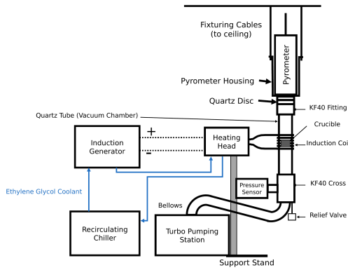
FIG. 1. System overview. The generator drives the liquid-cooled heating head/work coil around the vertically suspended quartz-tube chamber; the chamber stack is joined by KF40 flanges to the ceiling-suspended pyrometer housing, and an overpressure relief valve and flexible bellows lead past the pressure sensor to the turbo pumping station.
