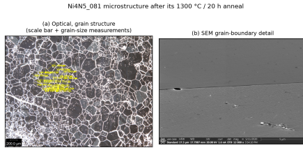
FIG. 5. Microstructure of a Ni4N5 specimen after a 1300\text{ }^{\circ}\text{C} / 20 h anneal under argon trickle flow. (a) Optical grain map with in-image grain-size measurements ( 200\mu\text{m} scale bar); (b) high-magnification SEM grain-boundary detail.
