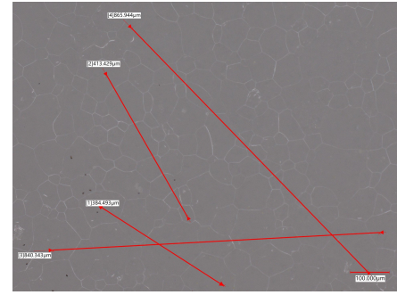
FIG. 6. As-recorded optical micrograph of the YSZ specimen after the 2500\text{ }^{\circ}\text{C} / 45 min tantalum-susceptor anneal, which coarsened the grains from \sim 20 to \sim 90\mu\text{m} . The red multi-grain measurement traces and the 100\mu\text{m} scale bar are part of the original microscope record.
