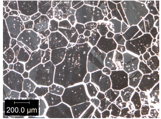
FIG. 6. Optical grain map of a Ni (4N5) specimen after a 1300 °C / 20 h anneal undergoing a constant 20 SCCM argon flow (200 μm scale bar), preceded by an evacuation of the chamber to high vacuum and a backfilling purge directly from high vacuum with argon. The equiaxed grain network is delineated by thermal grooving alone.
