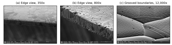
FIG. 5. Grain-boundary thermal grooving on a Ni (4N5) specimen after a 1200 °C / 12 h anneal, imaged edge-on in the as-annealed condition after only an ultrasonic ethanol clean. The grooves have deepened enough that they delineate the grain structure on their own. (a) Edge view at 350× (200 μm scale bar). Several grain boundaries traverse the full sheet thickness. (b) Edge and top surface at 800× (50 μm scale bar). The grooves outline the surface grain structure. (c) Grooved boundaries at 12,000× (5 μm scale bar). Multiple boundaries are grooved, and grooving is visible at several triple junctions. The trenches deepen as grain-boundary energy equilibrates against surface energy at the soak temperature.
