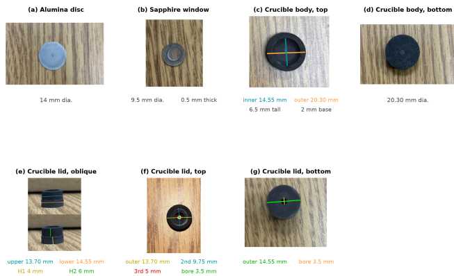
Figure 3: Measured dimensions of each part of the graphite crucible/susceptor stack, with the coloured measurement lines drawn on the corresponding photograph. (a) Alumina spacer disc, 14 mm dia. (b) Sapphire pyrometer window, 9.5 mm dia., 0.5 mm thick. (c) Crucible body, top: machined sample cavity 14.55 mm ID (teal), 20.30 mm OD (orange); the cup is 6.5 mm tall with a 2 mm base. (d) Crucible body, bottom face, 20.30 mm dia. (e) Crucible lid, oblique: the stepped plug seats into the cavity — 13.70 mm upper step (teal), 14.55 mm lower shoulder (orange); the upper step is 4 mm tall (H1, yellow) and the lower shoulder 6 mm tall (H2, green). (f) Crucible lid, top: four concentric steps of 13.70 mm (outermost), 9.75 mm, 5 mm, and a 3.5 mm central pyrometer-sighting bore. (g) Crucible lid, bottom: 14.55 mm seating face (green) and the 3.5 mm through-bore (orange). Two alumina discs sandwich the specimen inside the cavity, the lid seats on top, and the sapphire window closes the bore so the pyrometer sights the sample through the lid; fully assembled the stack stands 13 mm tall. Measurements contributed by R. Guymon.
