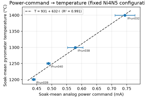
Figure 6: Power-command → temperature calibration for one fixed archived Ni4N5 configuration. Points are soak-mean values; horizontal bars are the in-soak SD of the analog command. The dashed line is a guide-to-the-eye linear fit ( R^2 = 0.991 , n = 4 ).
