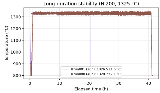
Figure 9: Long-duration thermal stability: Ni200 anneals at 1325 °C held for 20 h (IFRun081) and 40 h (IFRun080).
