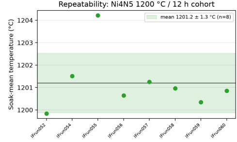
Figure 8: Run-to-run repeatability of the Ni4N5 1200 °C / 12 h cohort (IFRun052–IFRun060, n = 8 ). Points are per-run soak-mean temperatures; the band is mean \pm SD ( 1201.2 \pm 1.3 °C).
