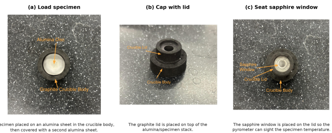
Figure 4: Specimen-loading sequence for the graphite crucible/susceptor, in order (orange call-outs name the visible parts). (a) The specimen is placed on an alumina sheet in the crucible body and covered with a second alumina sheet, so the alumina discs isolate the specimen from the graphite. (b) The graphite lid is seated on top of the alumina/specimen stack. (c) The sapphire window is placed over the lid bore, closing the crucible while leaving an optical path for the pyrometer to sight the specimen temperature through the window. Photographs contributed by R. Guymon.
