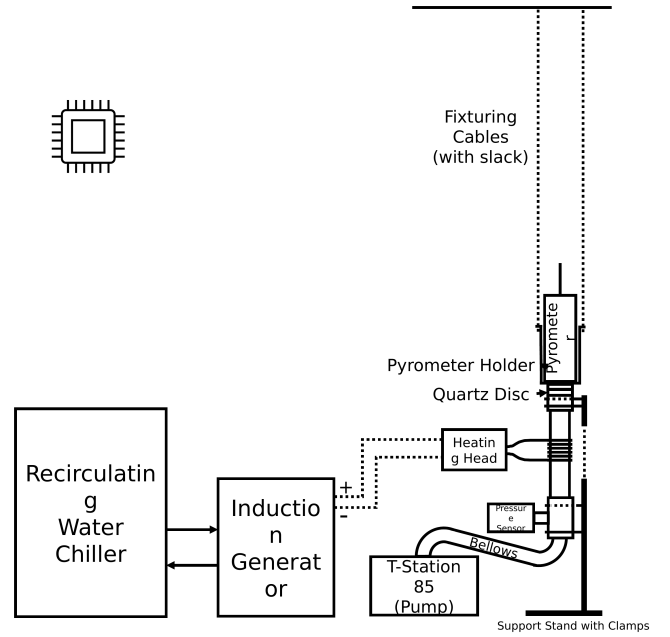
Figure 5: System overview of the computer-controlled, vacuum-integrated induction annealing system: recirculating water chiller and induction generator drive a water-cooled heating head/work coil around a quartz-tube vacuum chamber; a dual-wavelength pyrometer sights the charge through a quartz optical disc; an Edwards T-Station 85 turbo-molecular pump (with pressure gauge and bellows) evacuates the chamber; and a DAQ/laptop sets generator power and reads the pyrometer for closed-loop control. Rendered from the editable source schematic docs/induction-furnace-schematic.pptx.
