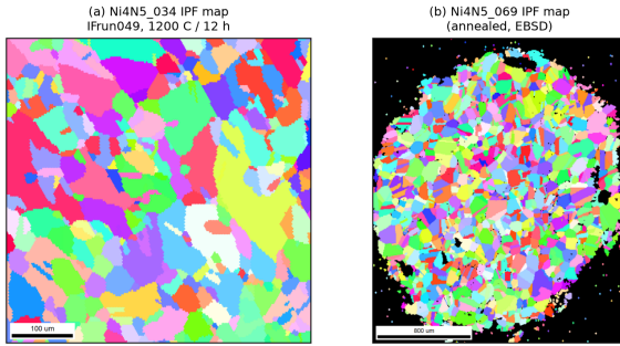
Figure 10: EBSD inverse-pole-figure (IPF) orientation maps of two annealed Ni4N5 specimens, rendered from the committed docs/SEM/ archive. (a) Ni4N5_034 (IFrun049, 1200 °C / 12 h); (b) Ni4N5_069. Each indexed color is a crystallographic orientation; the maps resolve hundreds of grains for grain-size and texture analysis.
