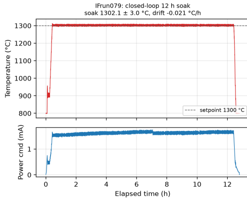
Figure 7: Representative closed-loop anneal (IFRun079, Ni4N5, nominal 1300 °C / 12 h): pyrometer temperature with setpoint overlay (top) and analog power command (bottom). Soak mean 1302.1 \pm 3.0 °C, drift -0.021 °C/h.
