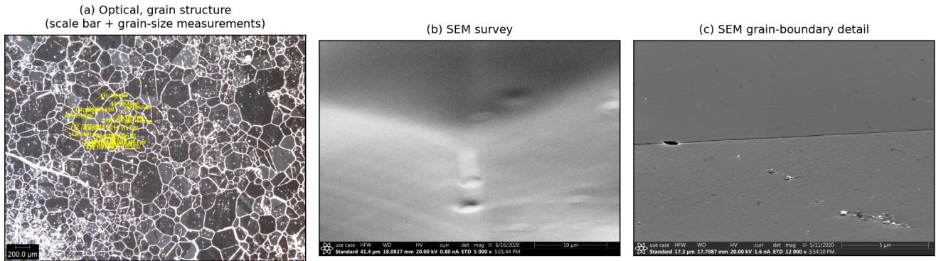
Figure 11: Multi-scale microstructure of specimen Ni4N5_081 after IFrun082 (nominal 1300 °C / 20 h, gas flow), correlating the characterization archive with a single logged thermal history. (a) Optical micrograph (grain structure, 200 μm scale bar, with in-image grain-size measurements); (b) SEM survey; (c) high-magnification SEM grain-boundary detail. All panels are committed files under docs/optical/ and docs/SEM/.
