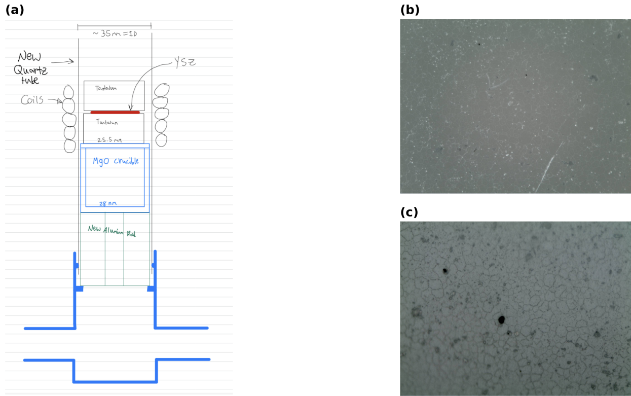
FIG. 18. High-temperature ceramic (YSZ) configuration and resulting microstructure. (a) Charge-stack schematic: inside a fresh \sim 35 mm-ID quartz tube, the YSZ specimen (red) is sandwiched between two 25.5 mm tantalum susceptor blocks, seated in a 28 mm MgO crucible on an alumina support rod that raises the stack to coil height; the coil, vacuum, pyrometer, and control paths are unchanged from the metal configuration. (b) Optical micrograph of YSZ after a 1700^\circ\text{C} / 10 h anneal. (c) Optical micrograph of an induction-annealed YSZ specimen, showing the equiaxed grain structure.
