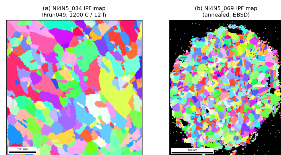
FIG. 13. EBSD inverse-pole-figure (IPF) orientation maps of two annealed Ni4N5 specimens, rendered from the archived EBSD scans. (a) Ni4N5_034 (IFrun049, 1200^\circ\text{C} / 12\text{h} ); (b) Ni4N5_069. Each indexed color is a crystallographic orientation; the maps resolve hundreds of grains for grain-size and texture analysis.
