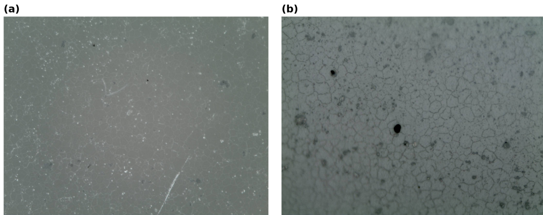
Figure S10: YSZ optical micrographs. (a) YSZ after a 1700 °C / 10 h anneal. (b) An induction-annealed YSZ specimen, showing the equiaxed grain structure. The tantalum-susceptor sample stack used for these anneals is drawn in the main text (Fig. 8).
