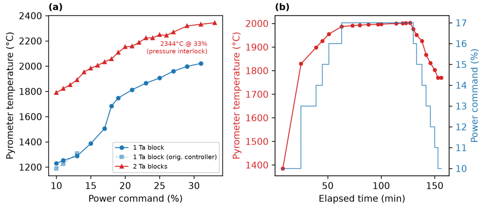
Figure S9: Measured heat curves of the tantalum-susceptor (ceramic) stack. (a) Pyrometer temperature vs. generator power command for one and two stacked tantalum susceptor blocks (the faint series repeats the single-block measurement on the original power controller); the two-block ramp reached 2344 °C at a 33 % command before the chamber pressure interlock ended the test. (b) Timed two-block ramp/soak: a constant 17 % command holds approximately 2000 °C ( 2000 \pm 3 °C over the final hour) before a stepped ramp-down.
