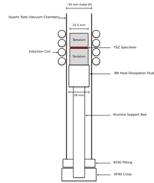
FIG. 8. Sample-stack configuration for the high-temperature ceramic anneals. The YSZ specimen is sandwiched between two 25.5\text{mm} tantalum susceptor blocks inside the quartz tube. The blocks rest on a boron nitride heat-dissipation stub, which sits on the alumina support rod that raises the sample stack to coil height. The coil, vacuum, pyrometer, and control paths are unchanged from the metal configuration.
