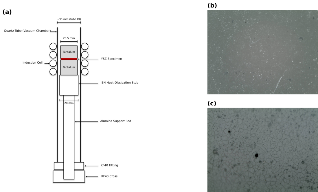
Figure S12: YSZ charge stack and resulting microstructure. (a) Charge-stack schematic: inside a fresh \sim 35 mm-ID quartz tube, the YSZ specimen (red) is sandwiched between two 25.5 mm tantalum susceptor blocks, resting on a 28 mm ceramic heat-dissipation stub (boron nitride for best results, sometimes MgO) on an alumina support rod that raises the stack to coil height; the coil, vacuum, pyrometer, and control paths are unchanged from the metal configuration. (b) Optical micrograph of YSZ after a 1700^{\circ}\text{C} / 10 h anneal. (c) Optical micrograph of an induction-annealed YSZ specimen, showing the equiaxed grain structure.
