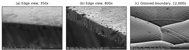
FIG. 5. Grain-boundary thermal grooving on a Ni4N5 specimen after a 1200^\circ\text{C} / 12 h anneal, imaged edge-on in the as-annealed condition after only an ultrasonic ethanol clean. (a) Edge view at 350\times ( 200\mu\text{m} scale bar). Several grain boundaries traverse the full sheet thickness. (b) Edge and top surface at 800\times ( 50\mu\text{m} scale bar). The grooves outline the surface grain structure. (c) A single grooved boundary at 12,000\times ( 5\mu\text{m} scale bar). The deep trench develops as grain-boundary energy equilibrates against surface energy at the soak temperature.
