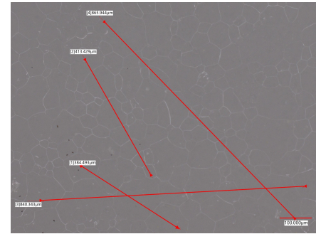
FIG. 7. As-recorded optical micrograph of the YSZ specimen after the 2500^\circ\text{C} / 45 min tantalum-susceptor anneal, which coarsened the grains from approximately 20 to 90\mu\text{m} . The red multi-grain measurement traces and the 100\mu\text{m} scale bar are part of the original microscope record.
