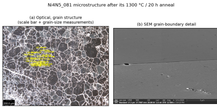
FIG. 5. Microstructure of a Ni4N5 specimen after a 1300 °C / 20 h anneal under a constant 20 SCCM argon flow. (a) Optical grain map with in-image grain-size measurements (200 \mu\text{m} scale bar); (b) high-magnification SEM grain-boundary detail.
