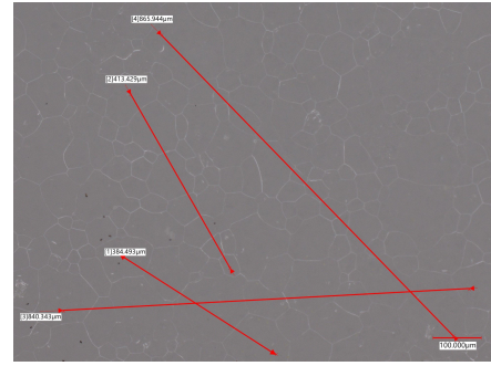
FIG. 6. As-recorded optical micrograph of the YSZ specimen after the 2500 °C / 45 min tantalum-susceptor anneal, which coarsened the grains from approximately 20 to 90 \mu\text{m} . The red multi-grain measurement traces and the 100 \mu\text{m} scale bar are part of the original microscope record.
