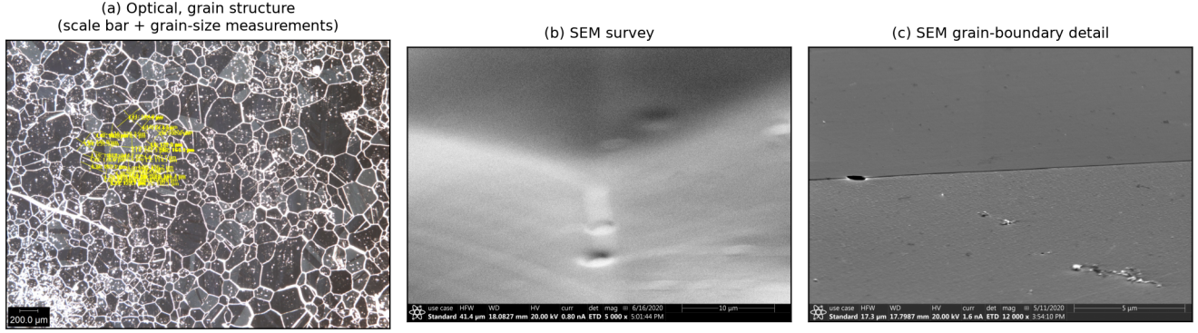
Figure 6: Multi-scale microstructure of specimen Ni4N5_081 after IFrun082 (nominal 1300 °C / 20h, gas flow), correlating the characterization archive with a single logged thermal history. (a) Optical micrograph (grain structure, 200µm scale bar, with in-image grain-size measurements); (b) SEM survey; (c) high-magnification SEM grain-boundary detail. All panels are committed files under docs/optical/ and docs/SEM/.
