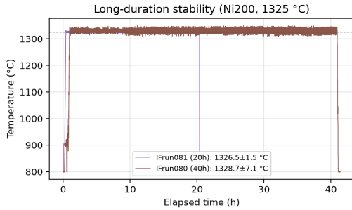
Figure 4: Long-duration thermal stability: Ni200 anneals at 1325 °C held for 20 h (IFrun081) and 40 h (IFrun080).
