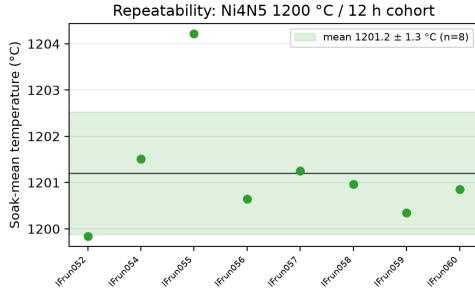
Figure 3: Run-to-run repeatability of the Ni4N5 1200 °C / 12 h cohort (IFrun052–IFrun060, n = 8 ). Points are per-run soak-mean temperatures; the band is mean \pm SD ( 1201.2 \pm 1.3\text{ }^{\circ}\text{C} ).
