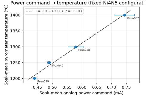
Figure 1: Power-command → temperature calibration for one fixed archived Ni4N5 configuration. Points are soak-mean values; horizontal bars are the in-soak SD of the analog command. The dashed line is a guide-to-the-eye linear fit ( R^2 = 0.991 , n = 4 ).
