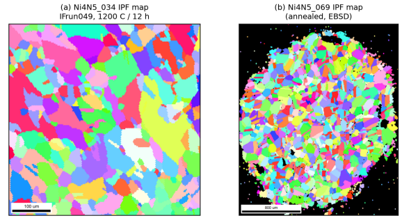
Figure 5: EBSD inverse-pole-figure (IPF) orientation maps of two annealed Ni4N5 specimens, rendered from the committed docs/SEM/ archive. (a) Ni4N5_034 (IFrun049, 1200 °C / 12 h); (b) Ni4N5_069. Each indexed color is a crystallographic orientation; the maps resolve hundreds of grains for grain-size and texture analysis.
