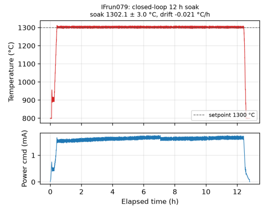
Figure 2: Representative closed-loop anneal (IFRun079, Ni4N5, nominal 1300 °C / 12 h): pyrometer temperature with setpoint overlay (top) and analog power command (bottom). Soak mean 1302.1 \pm 3.0 °C, drift -0.02 °C/h.
