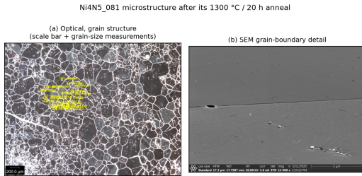
FIG. 4. Microstructure of specimen Ni4N5.081 after its logged anneal (nominal 1300^\circ\text{C} / 20 h, gas flow). (a) Optical grain map with in-image grain-size measurements (200 \mu\text{m} scale bar); (b) high-magnification SEM grain-boundary detail.
