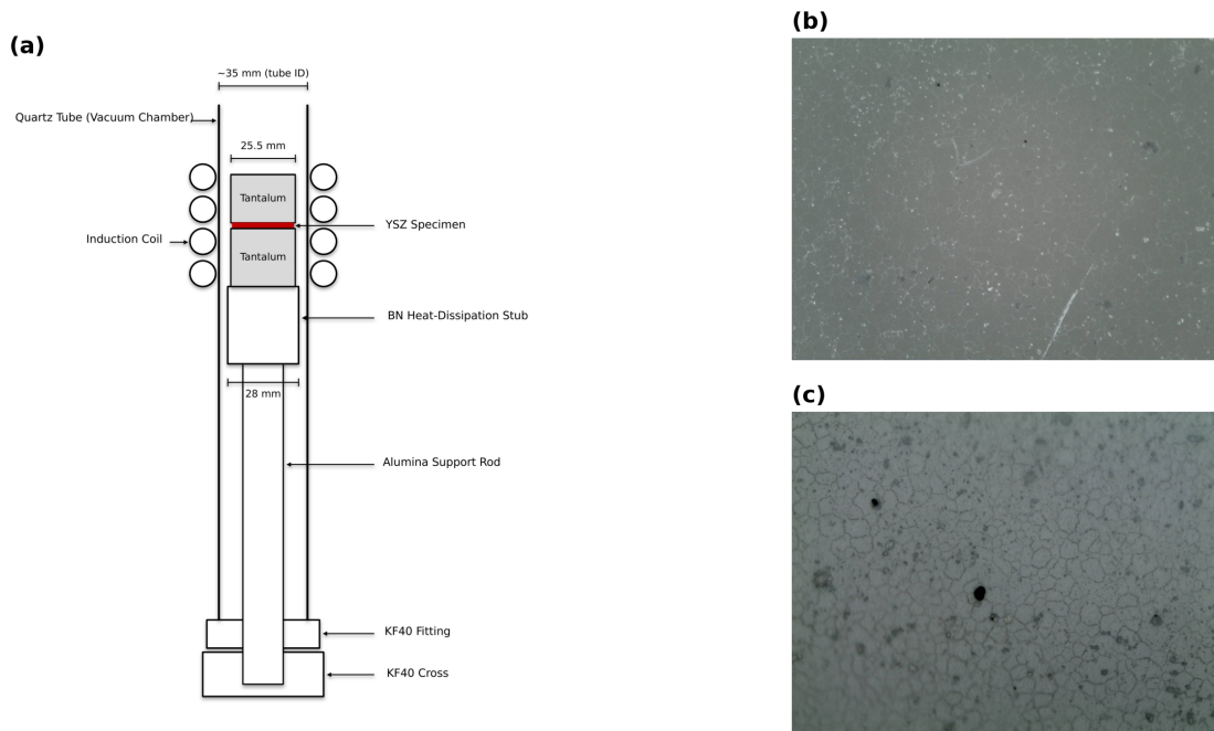
Figure S13: YSZ charge stack and resulting microstructure. (a) Charge-stack schematic: inside a fresh ~35 mm-ID quartz tube, the YSZ specimen (red) is sandwiched between two 25.5 mm tantalum susceptor blocks, resting on a 28 mm ceramic heat-dissipation stub (boron nitride for best results, sometimes MgO) on an alumina support rod that raises the stack to coil height; the coil, vacuum, pyrometer, and control paths are unchanged from the metal configuration. (b) Optical micrograph of YSZ after a 1700 °C / 10 h anneal. (c) Optical micrograph of an induction-annealed YSZ specimen, showing the equiaxed grain structure.
