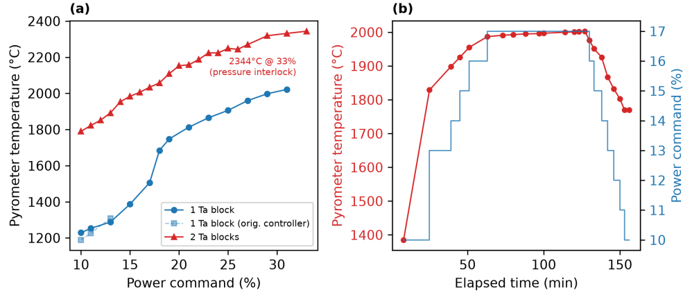
Figure S12: Measured heat curves of the tantalum-susceptor (ceramic) stack. (a) Pyrometer temperature vs. generator power command for one and two stacked tantalum susceptor blocks (the faint series repeats the single-block measurement on the original power controller); the two-block ramp reached 2344 °C at a 33% command before the chamber pressure interlock ended the test. (b) Timed two-block ramp/soak: a constant 17% command holds ~2000 °C ( 2000 \pm 3 °C over the final hour) before a stepped ramp-down.
