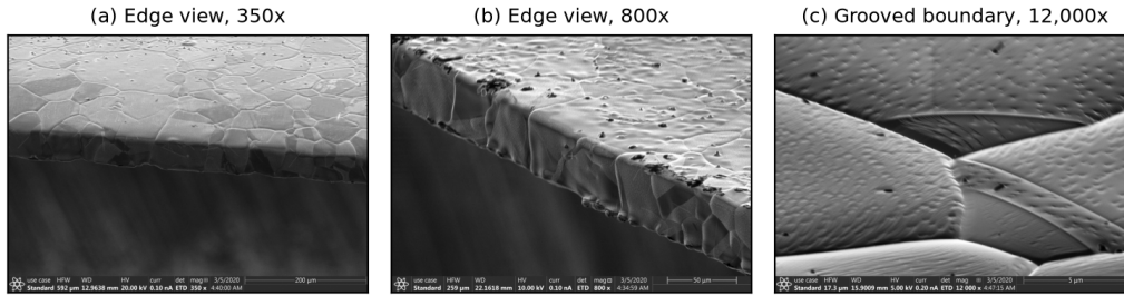
Figure S11: Grain-boundary thermal grooving on specimen Ni4N5.053 after a 1200 °C / 12 h anneal, imaged edge-on in the as-annealed condition (ultrasonic ethanol clean only; no polishing). (a) Edge view at 350 \times (200 \mu m scale bar): several grain boundaries traverse the full sheet thickness. (b) Edge and top surface at 800 \times (50 \mu m scale bar), with grooves outlining the surface grain structure. (c) A single grooved boundary at 12,000 \times (5 \mu m scale bar): the deep trench develops as grain-boundary energy equilibrates against surface energy at the soak temperature.
