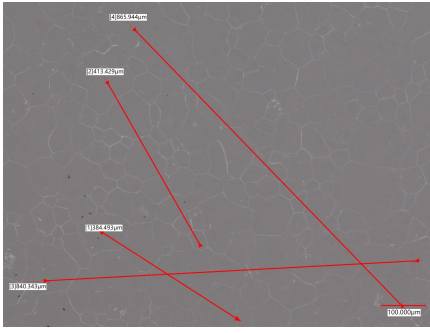
FIG. 10. As-recorded optical micrograph of the YSZ specimen after the 2500 °C / 45 min tantalum-susceptor anneal, which coarsened the grains from approximately 20 to 90 \mu\text{m} . The red multi-grain measurement traces and the 100 \mu\text{m} scale bar are part of the original microscope record.
