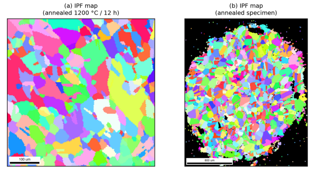
FIG. 7. EBSD inverse-pole-figure (IPF) orientation maps of two furnace-annealed Ni4N5 specimens, rendered from the recorded EBSD scans. (a) A specimen annealed at 1200^\circ\text{C} for 12 h ( 100\mu\text{m} scale bar). (b) A second annealed specimen ( 800\mu\text{m} scale bar). The maps resolve hundreds of grains for grain-size and texture analysis.
