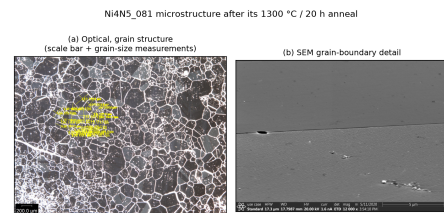
FIG. 9. Microstructure of a Ni4N5 specimen after a 1300^\circ\text{C} / 20 h anneal under a constant 20 SCCM argon flow. (a) Optical grain map with in-image grain-size measurements ( 200\mu\text{m} scale bar); (b) high-magnification SEM grain-boundary detail.
